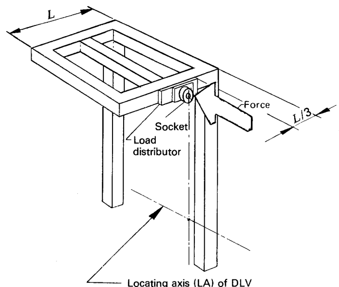
Figure 5d) — Load-distribution device for ROPS with two-post system
