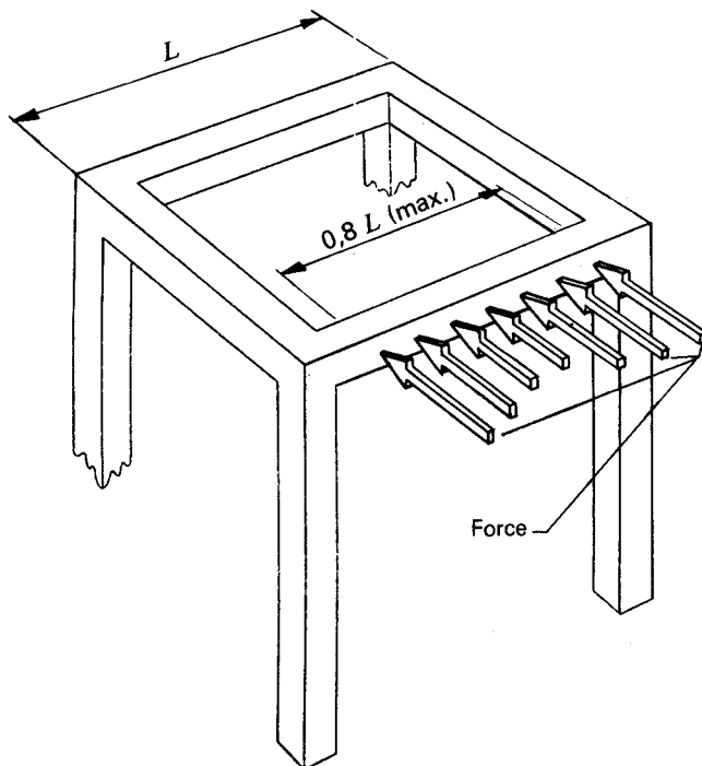
Figure 5a) — Load-distribution device for ROPS with four-post system
