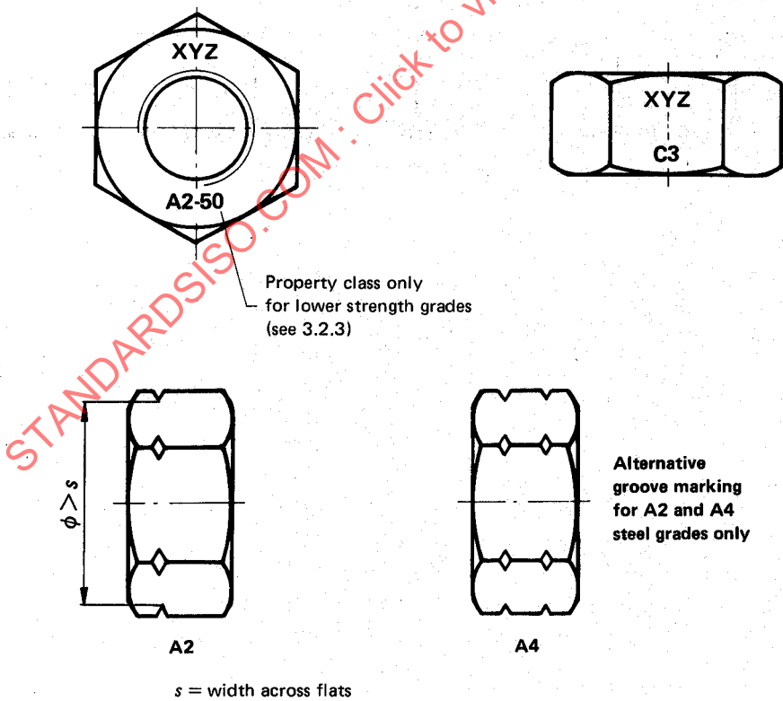
FIGURE 2 — Marking of nuts — Examples of alternative marking practice
