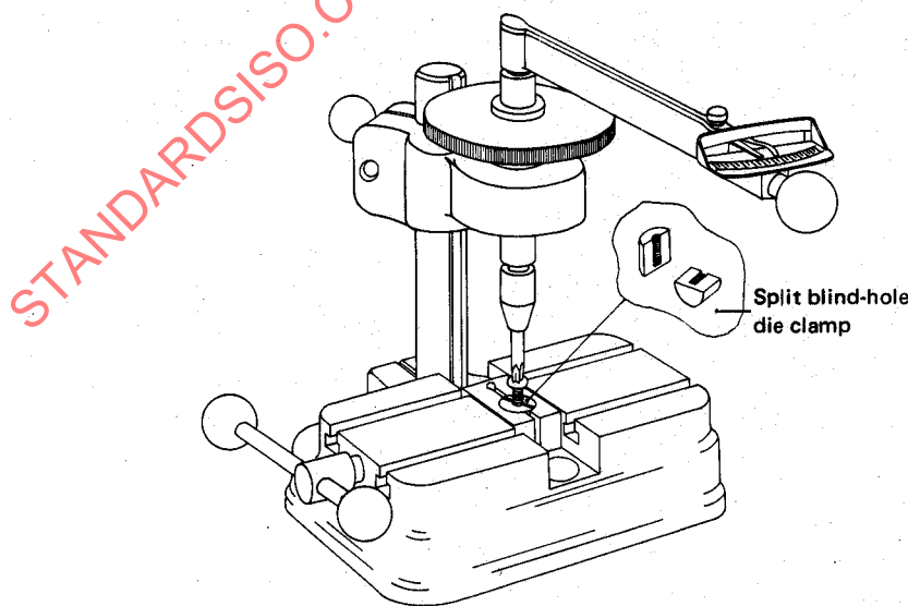
FIGURE 6 — Apparatus for determination of breaking torque ( T_m ) (see 6.5)
