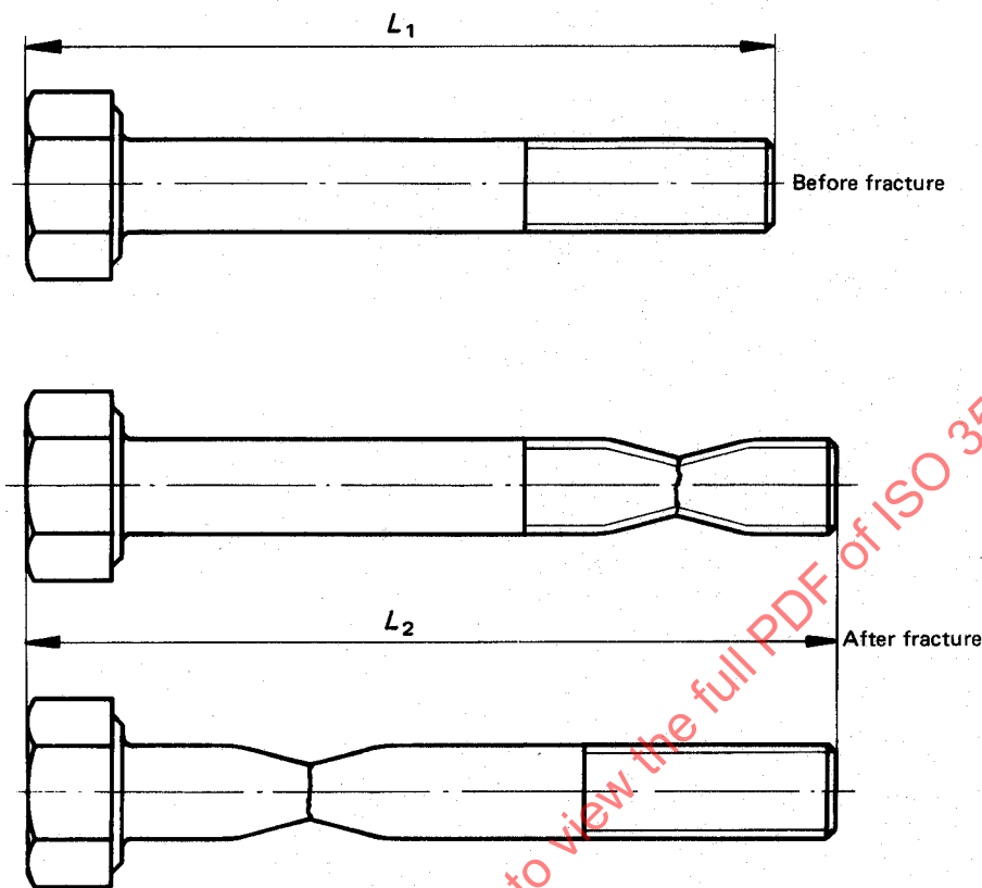
FIGURE 5 — Determination of total extension at fracture ( A_L ) (see 6.4)
