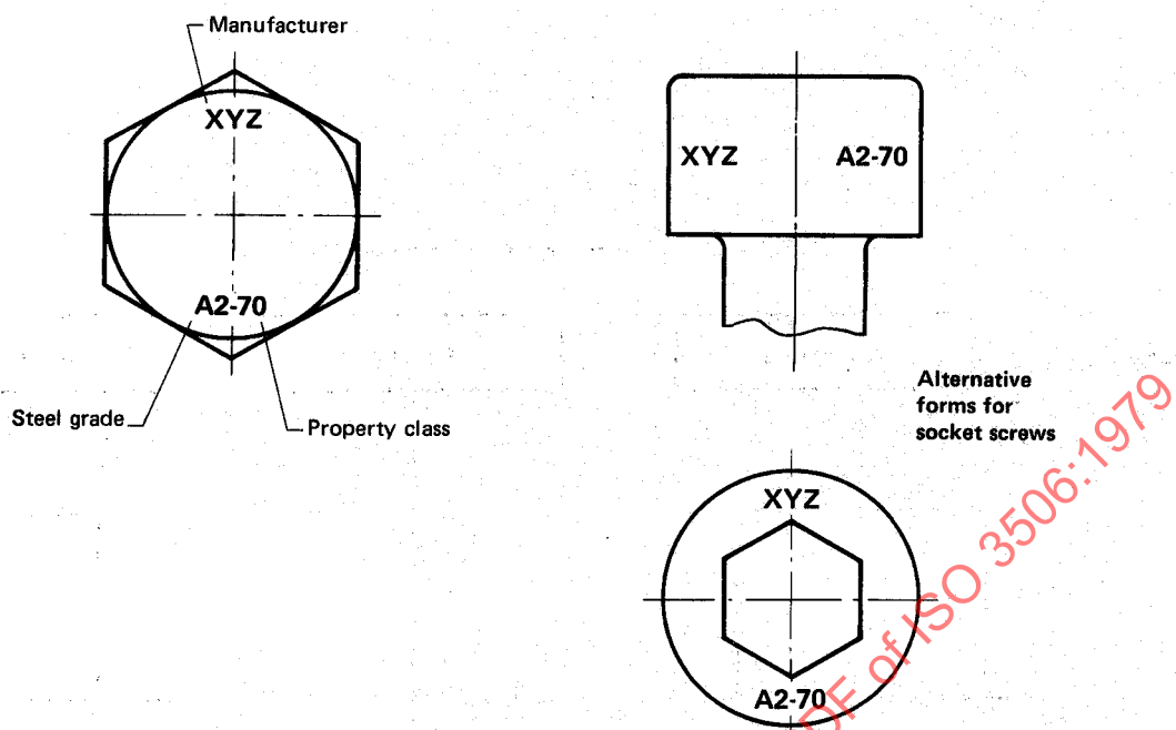
FIGURE 1 — Marking of bolts and screws — Examples
