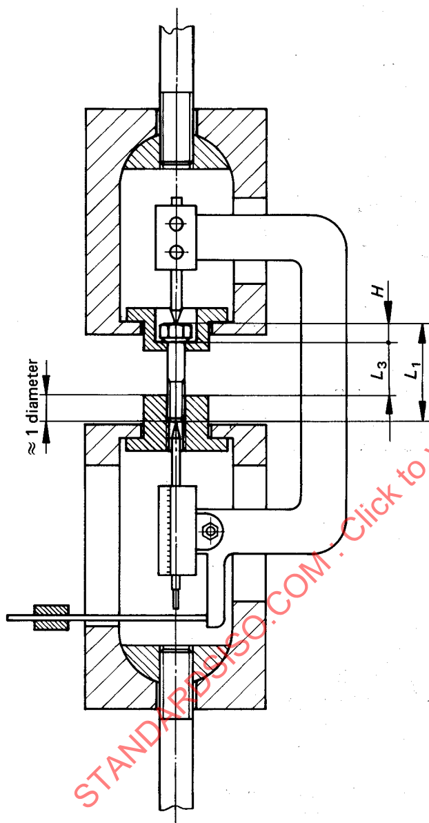
FIGURE 3 — Bolt extensometer with self-aligning grips
