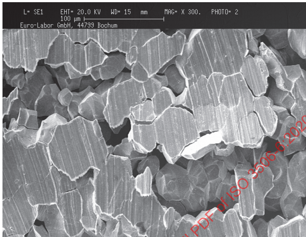
Figure 2 — Intergranular corrosion on a stainless steel 4301-304-00-I with 0,036 % C
