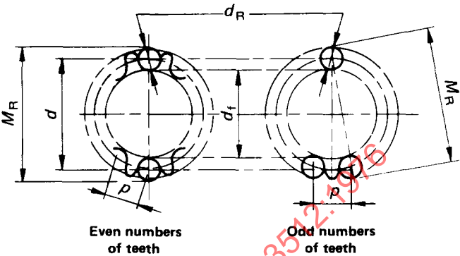
FIGURE 4 — Diametral dimensions
