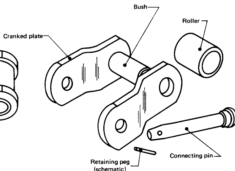
FIGURE 2 — Typical cranked link components
