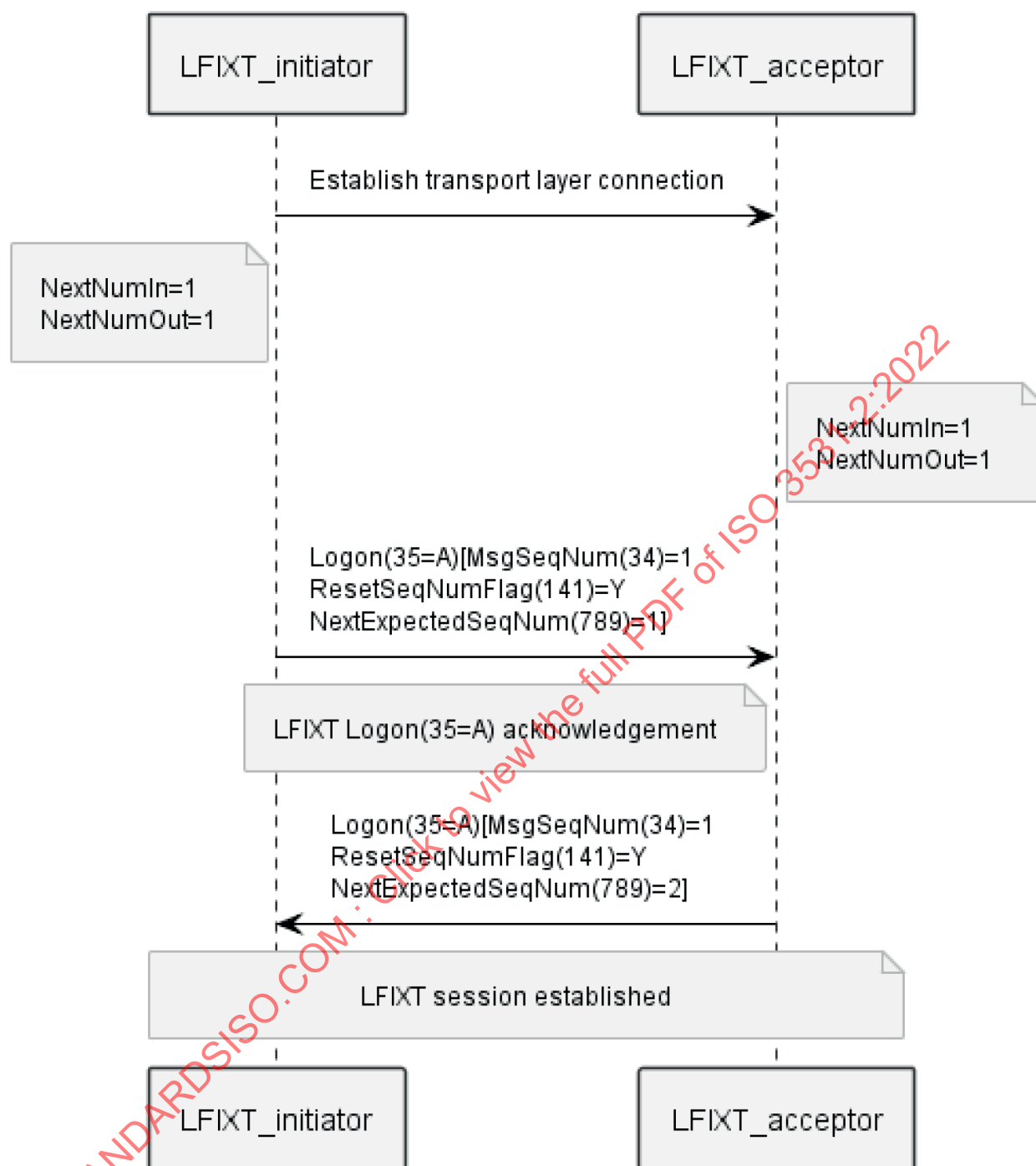
Figure 21 — LFIXT logon process
