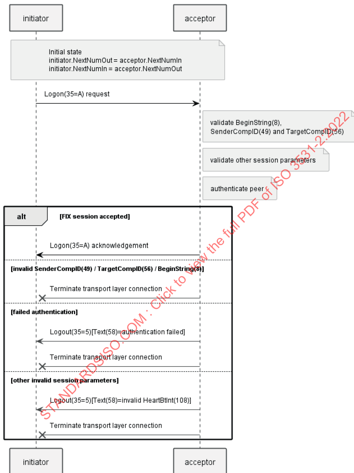
Figure 2 — FIX connection establishment
