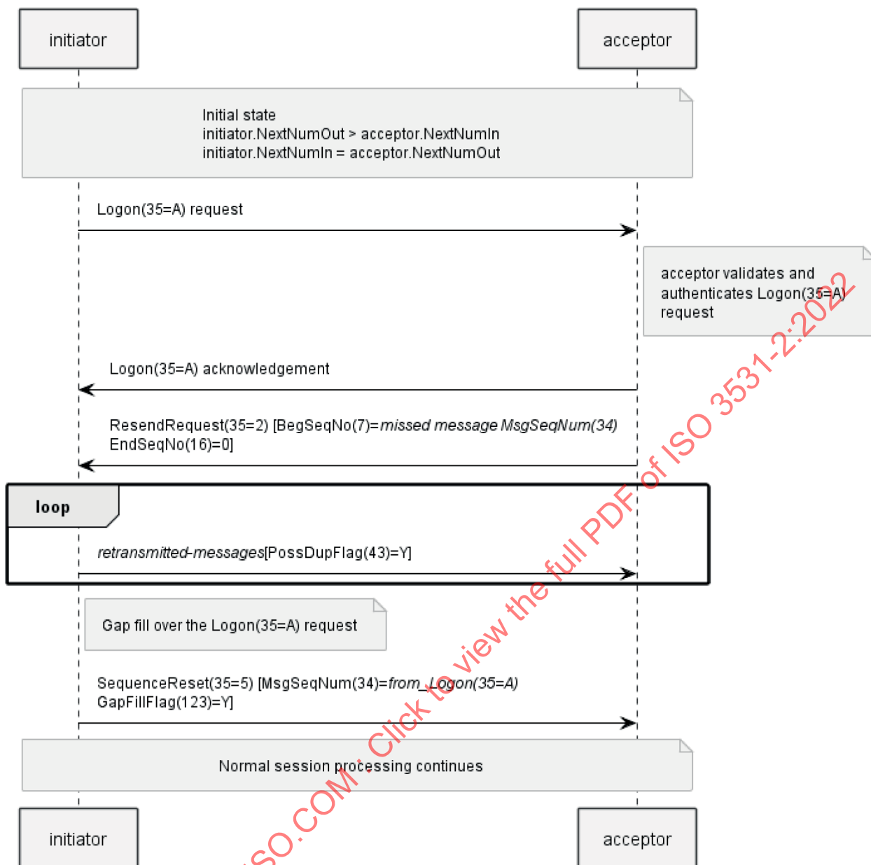
Figure 3 — ResendRequest(35=2) sent by acceptor after Logon(35=A) acknowledgement
