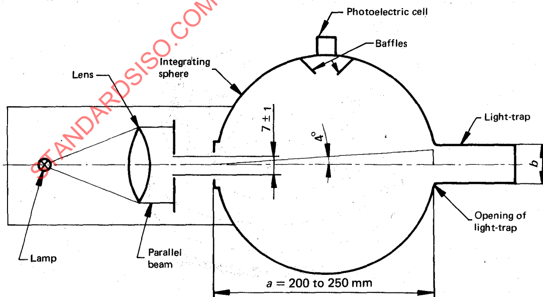
FIGURE 3 – Hazemeter
