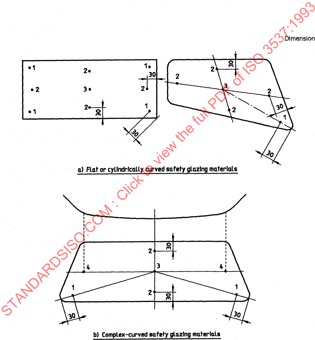
Figure 4 — Impact points
