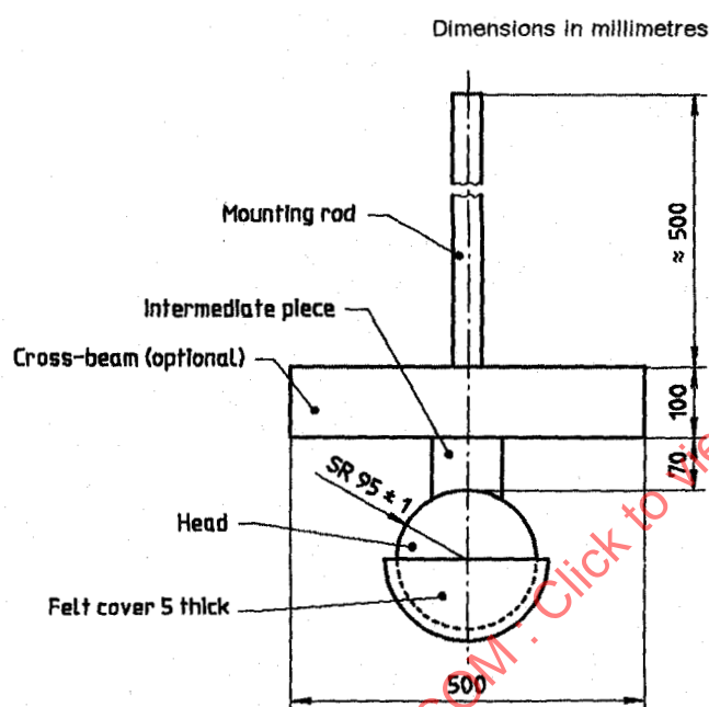
Figure 5 — Head-form weight
