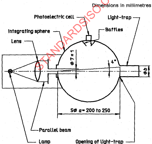
Figure 3 — Hazemeter
