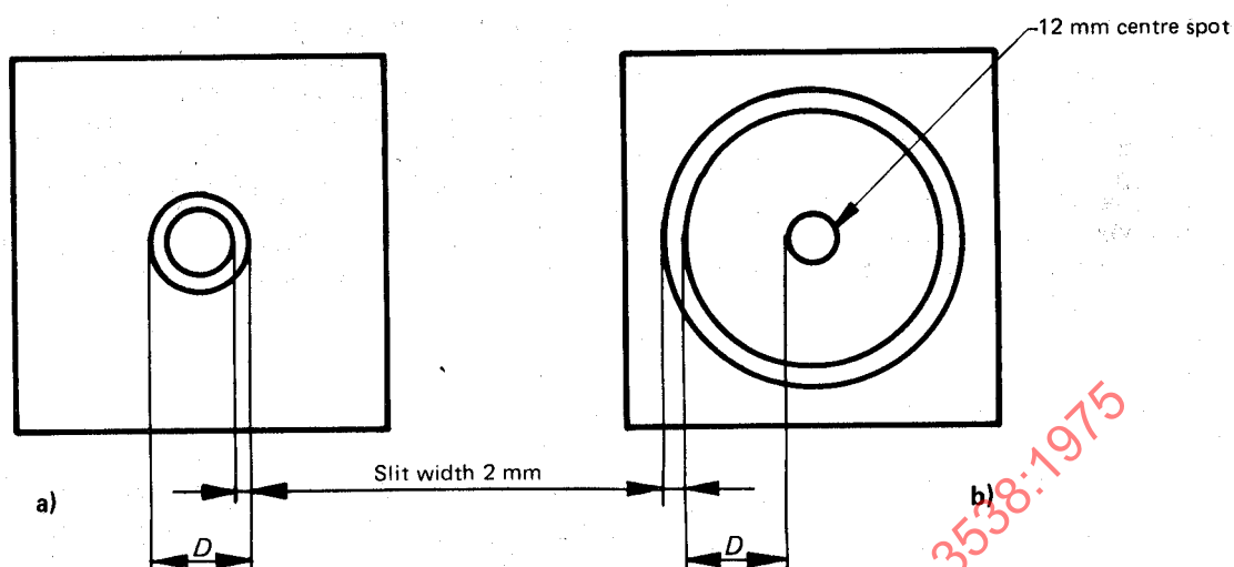
FIGURE 1 — Dimensions of targets
