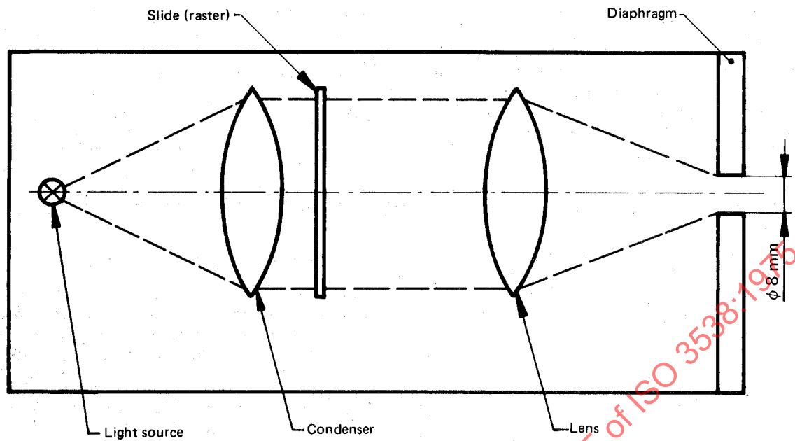
FIGURE 6 — Optical arrangement of the projector
