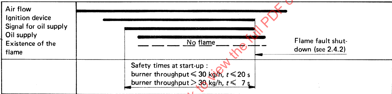
Diagram with flame fault shut-down at start-up
