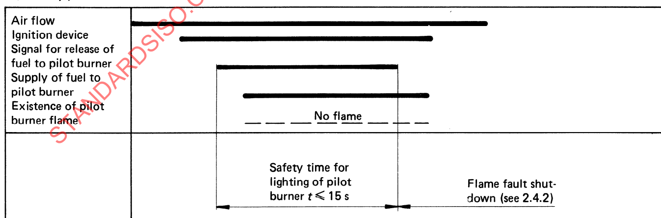
Diagrams with safety shut-down at start-up
