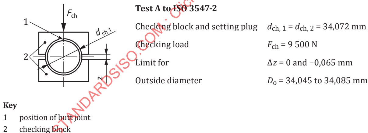
Figure 2 — Example of presentation of data on drawing
