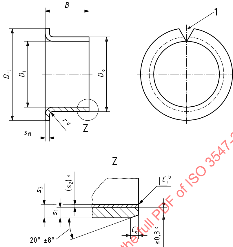
b) Type F flanged bush
