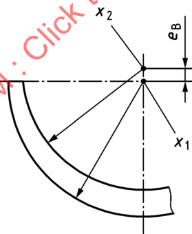
Figure 3 — Eccentric bearing bore of half bearing
