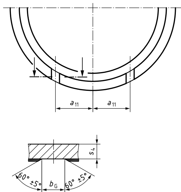
Figure 16 — Groove form on the flange face
