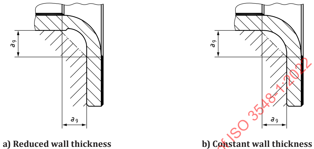
Figure 11 — Types of transition between radial parts of the flange
