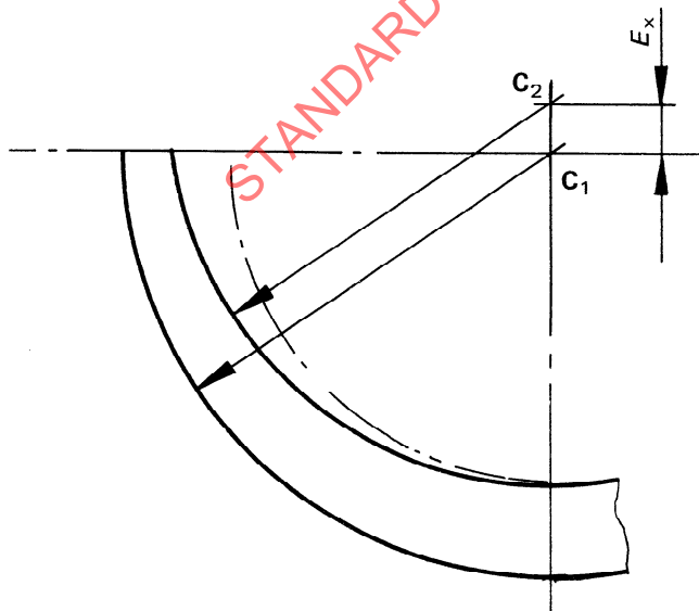
FIGURE 4 — Eccentric bore
