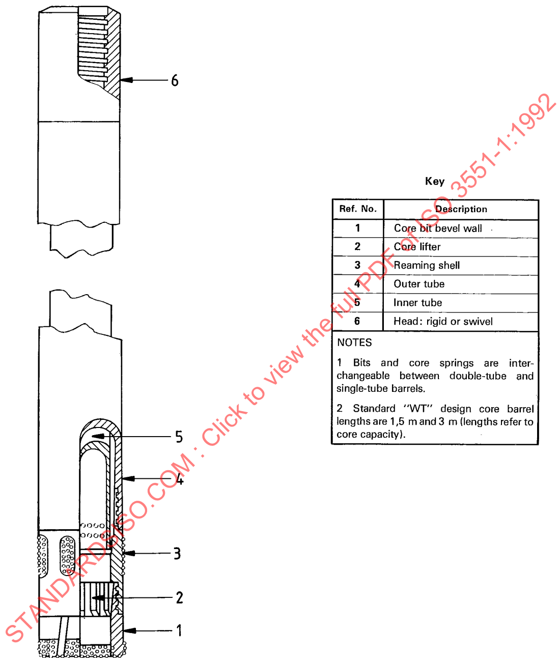
Figure 48 — "WT" design double-tube core barrel — Assembly — Rigid and swivel types BWT, NWT and HWT
