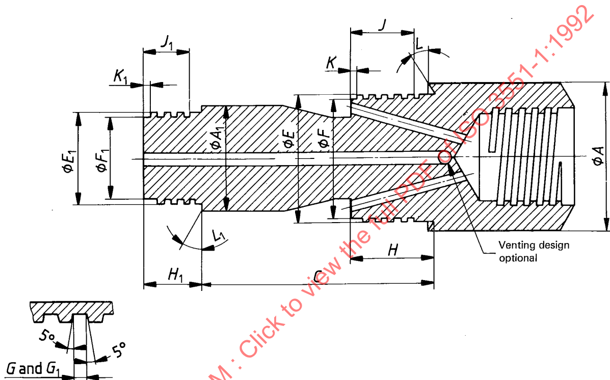
Figure 44 — “WM” design double-tube core barrel — Head (see table 42)
