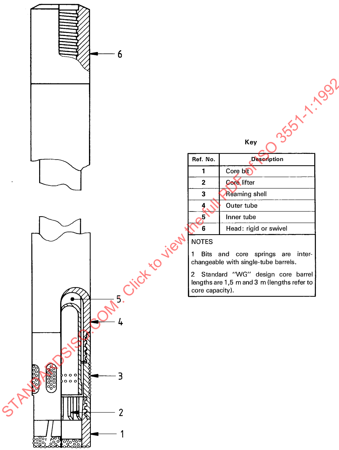
Figure 32 — "WG" design double-tube core barrel — Assembly — Rigid and swivel types
