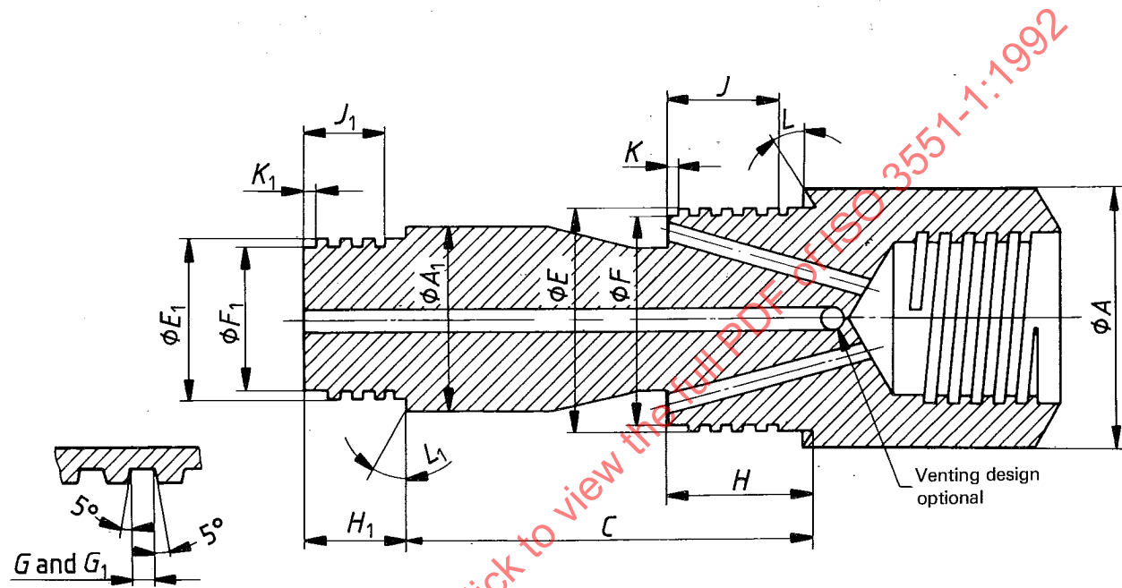
Figure 36 — “WG” design double-tube core barrel — Head (see table 35)
