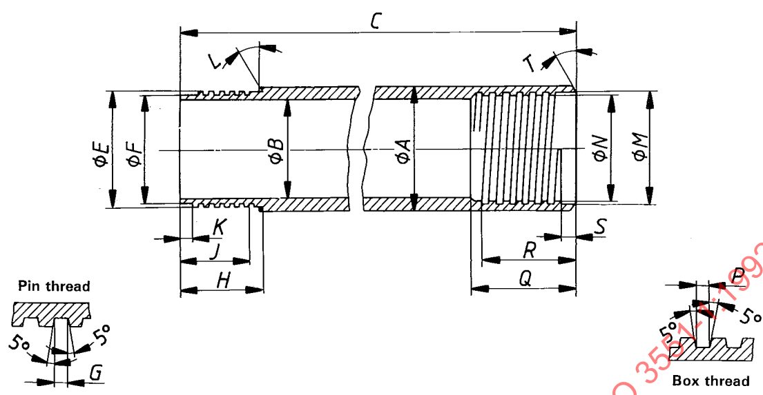
Figure 24 — “WF” design double-tube core barrel — Outer tube (see table 25)
