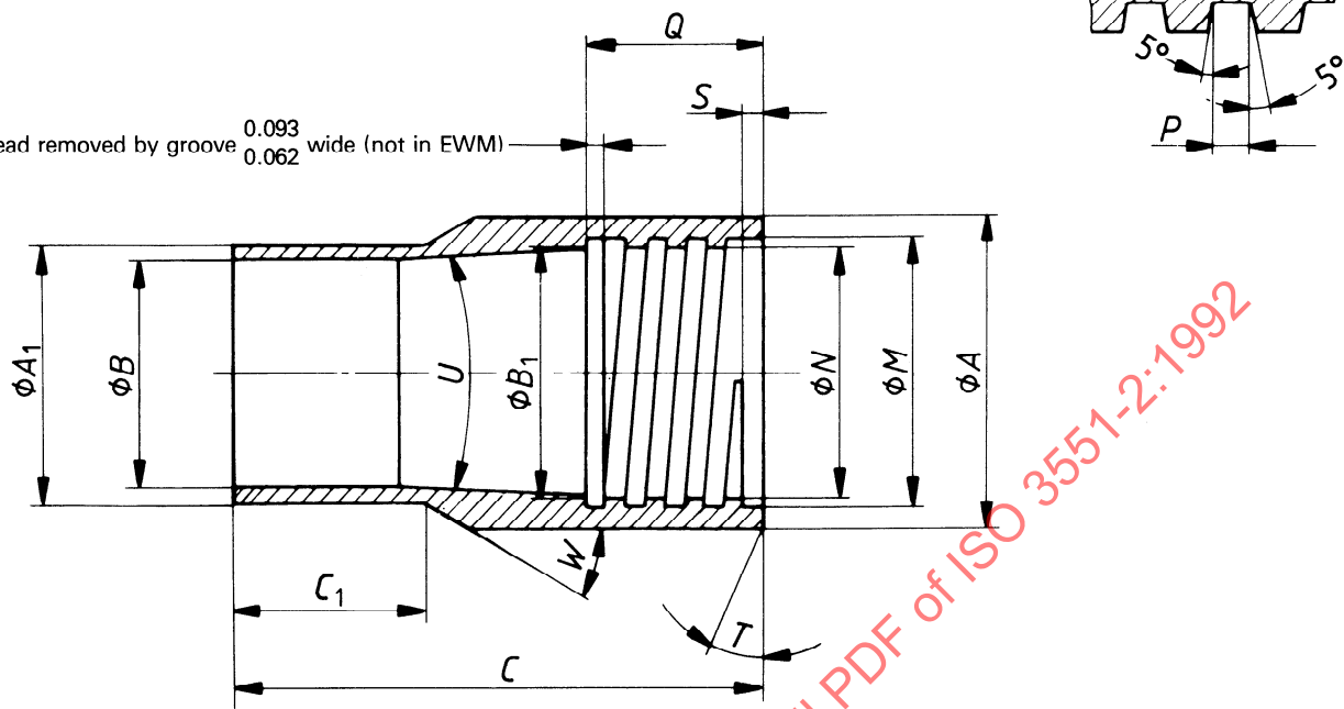
Figure 39 — "WM" design double-tube core barrel — Core-lifter case (see table 37)
