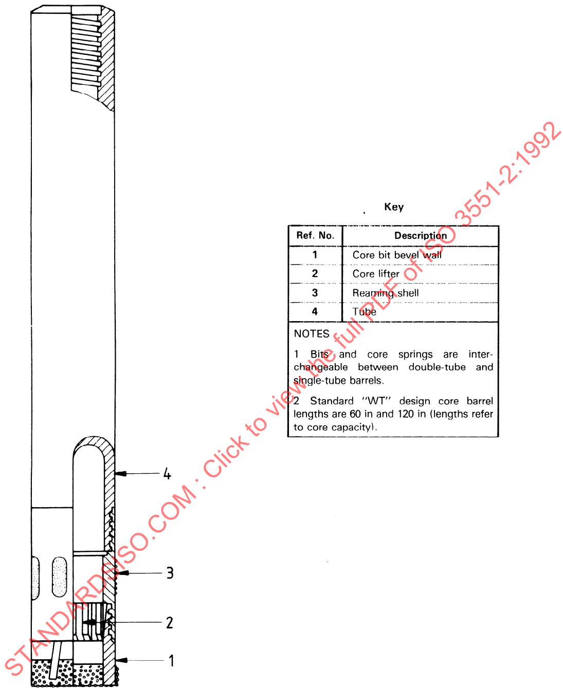
Figure 45 — "WT" design single-tube core barrel — Assembly — Sizes BWT, NWT and HWT
