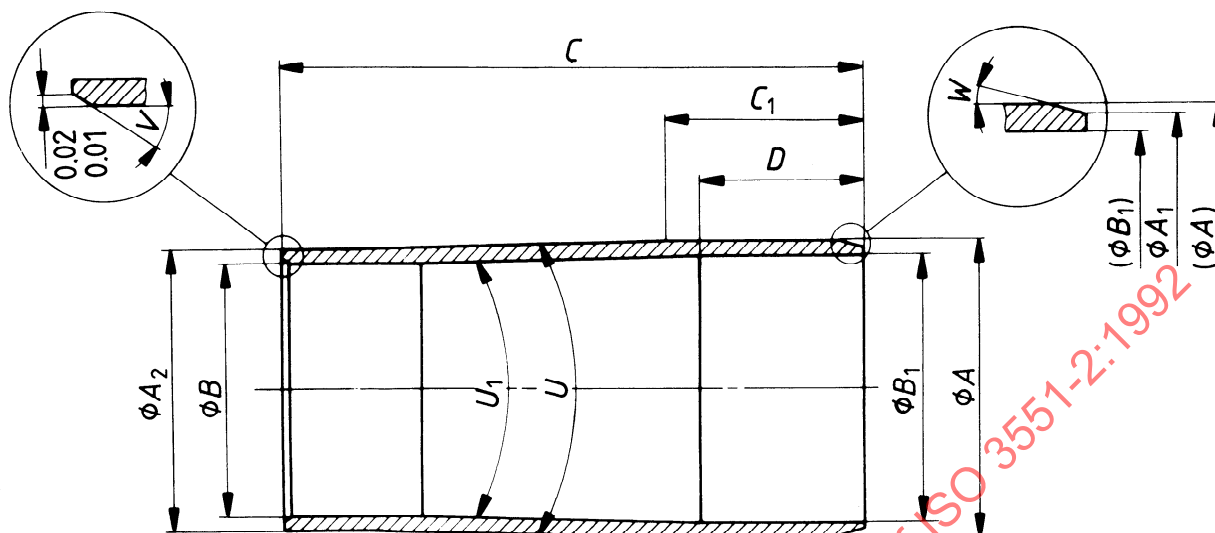
Figure 21 — "WF" design double-tube core barrel — Core-lifter case (see table 22)
