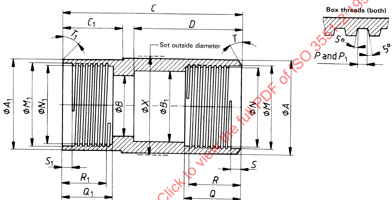
Figure 33 – “WG” design double-tube core barrel – Reaming shell (see table 32)
