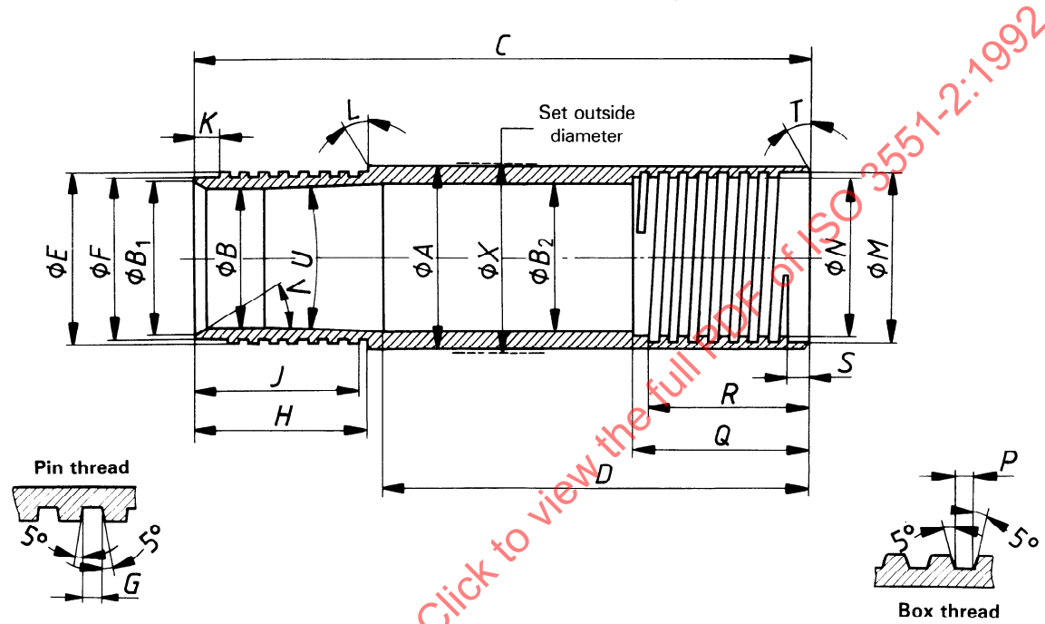
Figure 23 — “WF” design double-tube core barrel — Reaming shell (see table 24)
