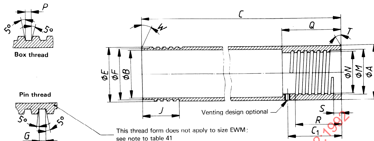
Figure 43 — "WM" design double-tube core barrel — Inner tube (see table 41)
