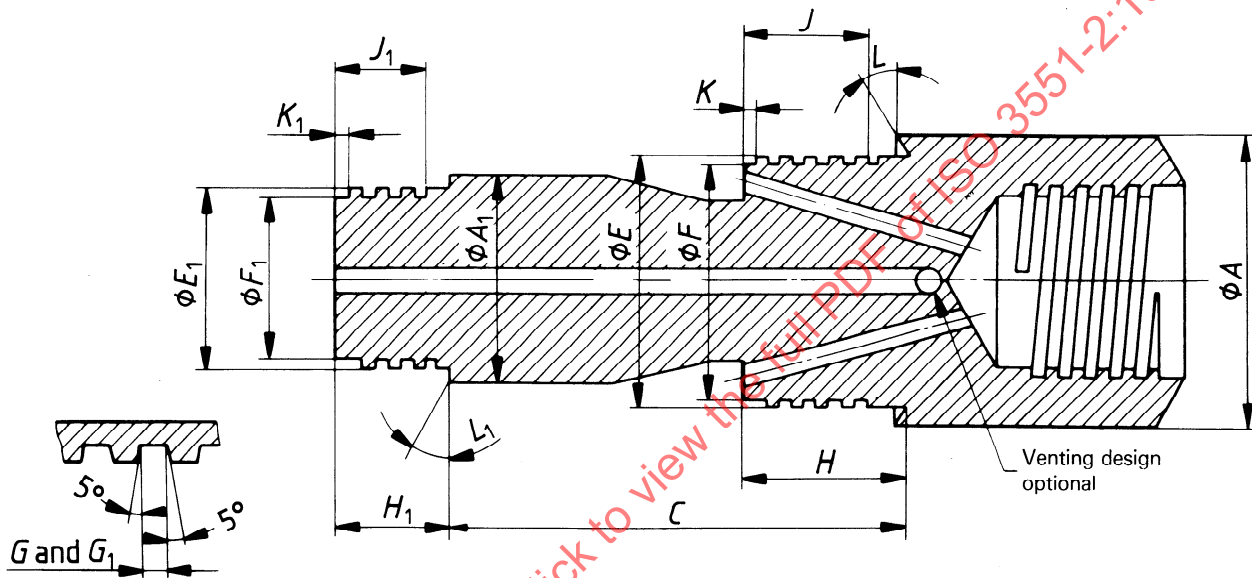
Figure 36 — “WG” design double-tube core barrel — Head (see table 35)
