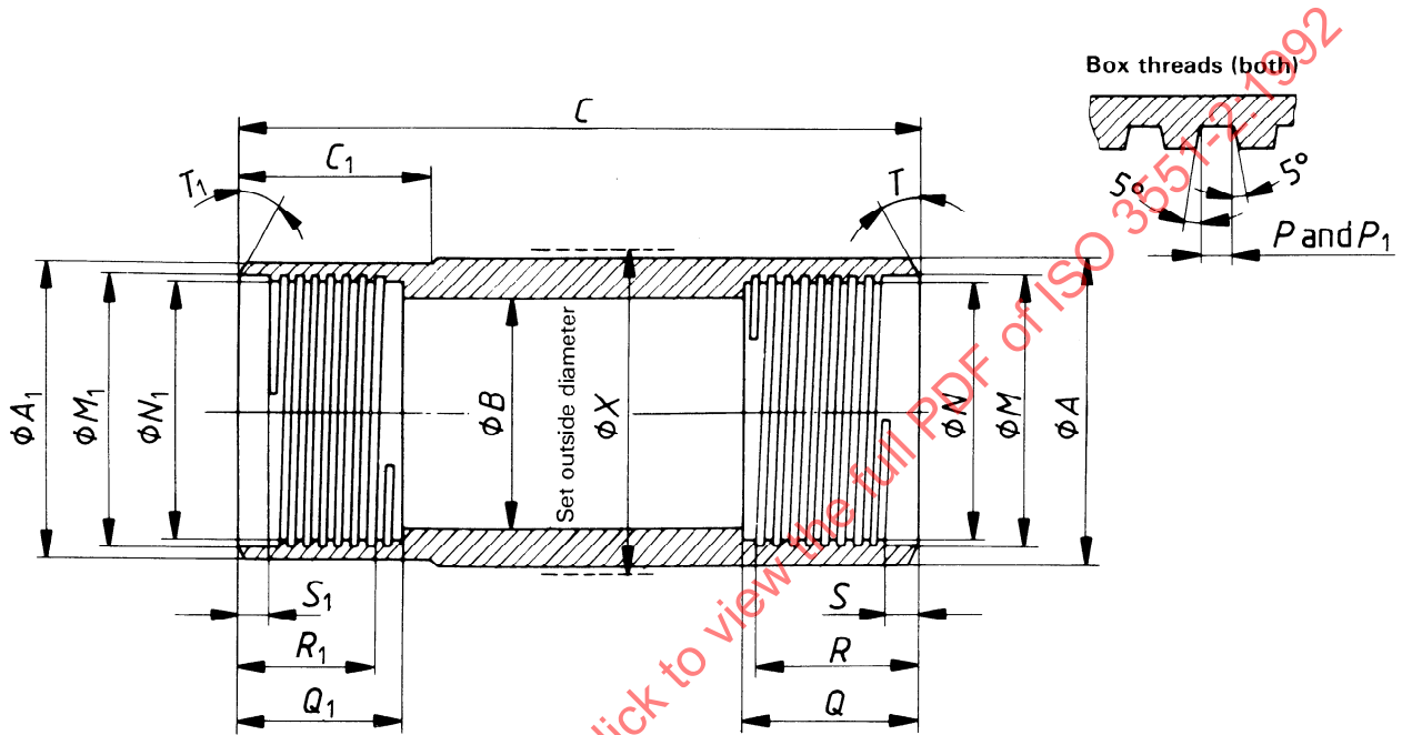
Figure 51 — "WT" design double-tube core barrel — Reaming shell (see table 47)
