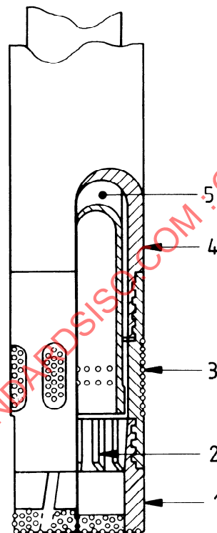
Figure 32 — "WG" design double-tube core barrel — Assembly — Rigid and swivel types
