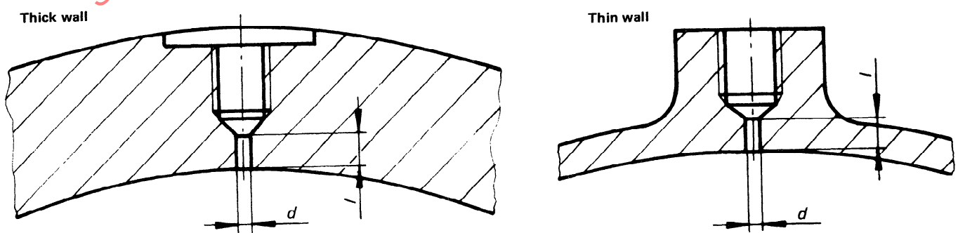
FIGURE 5 — Requirements for static head tapings
