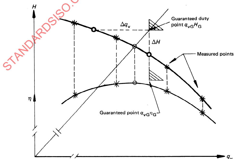
FIGURE 11 — Curve q_v H for the verification of the guarantee
