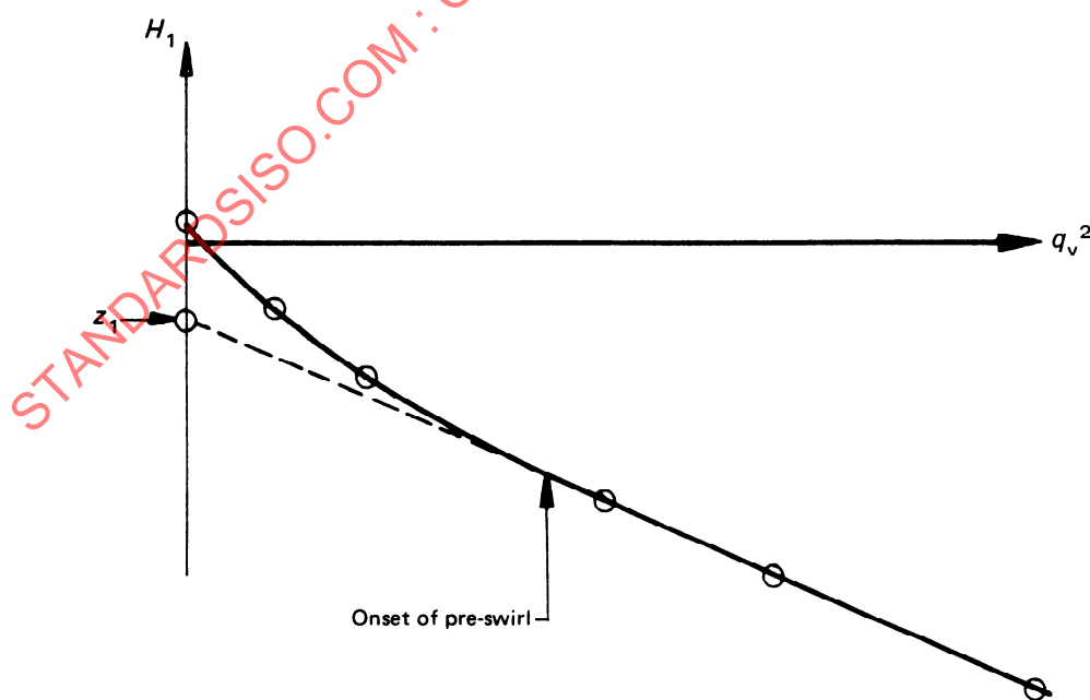
FIGURE 13 — Correction of measured inlet head
