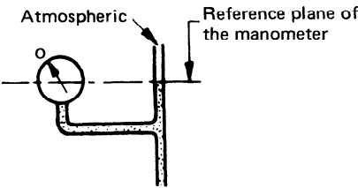
a) Arrangement for determining reference plane of Bourdon type gauge
