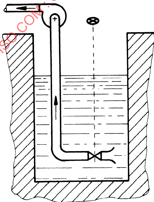
FIGURE 9 – Cavitation tests – Variation of (NPSH) by means of a throttle valve at inlet
