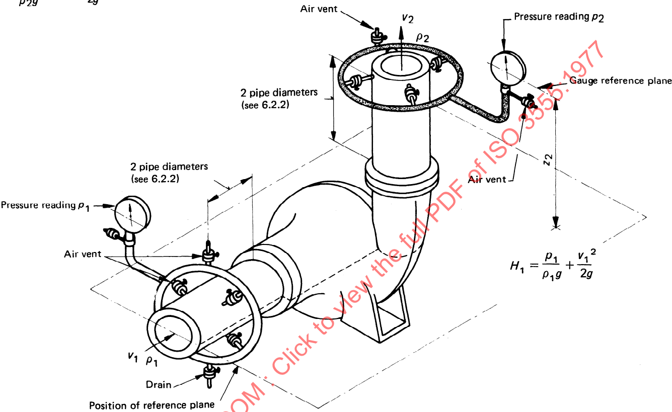
b) The pump inlet is under vacuum
