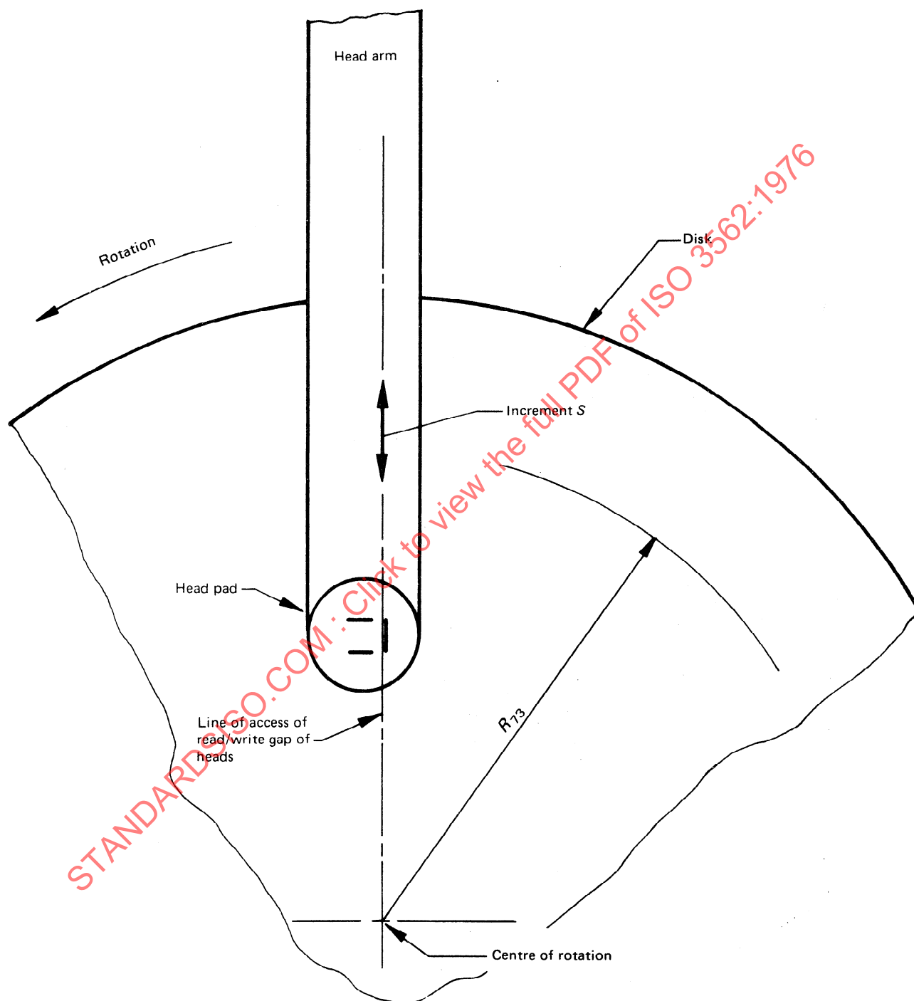
FIGURE 13 — Geometry of the head disk system
