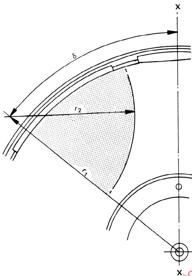
FIGURE 7 — Part of figure 6 with the brush area
