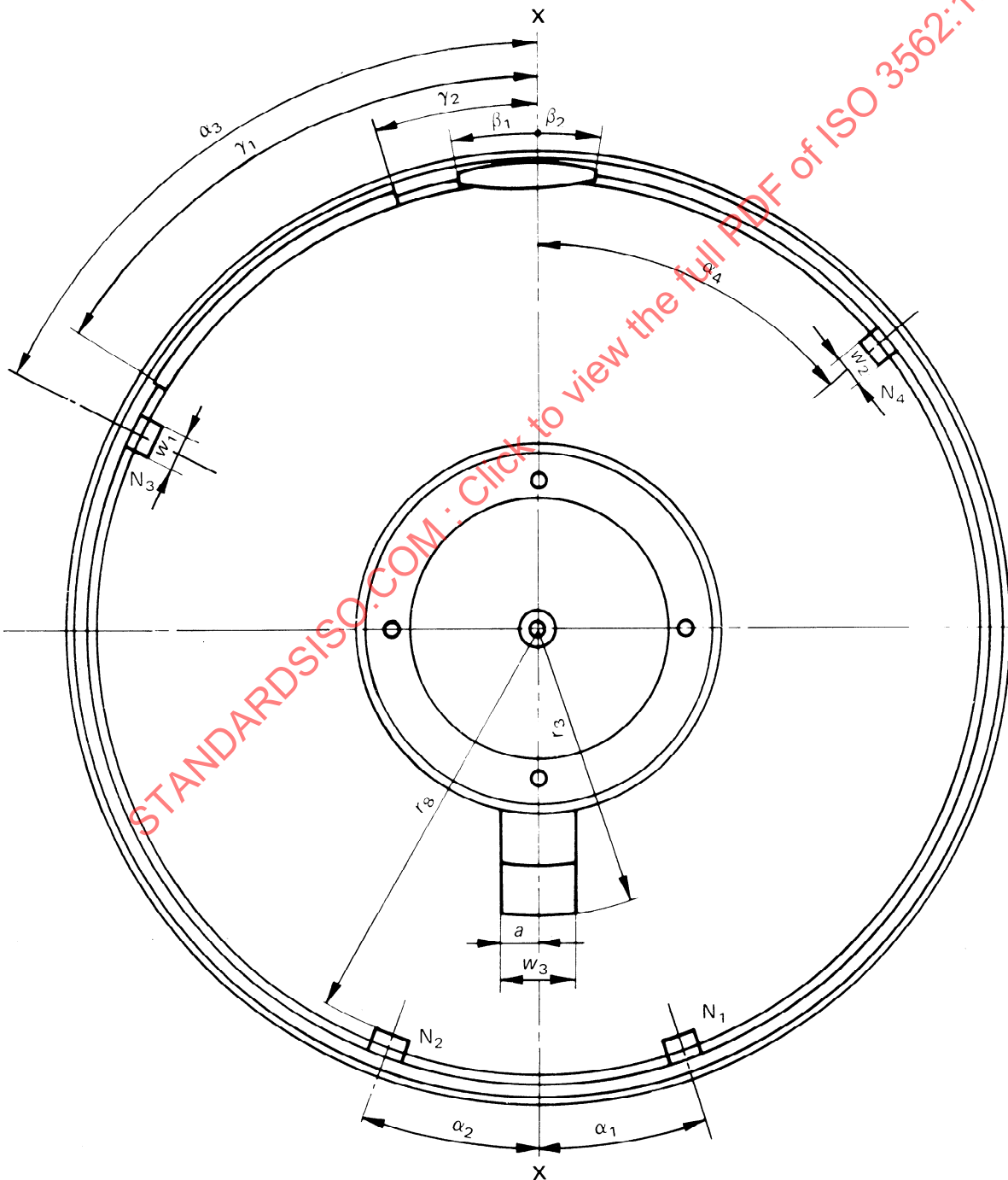
FIGURE 6 – View in direction of arrow A in figure 5
