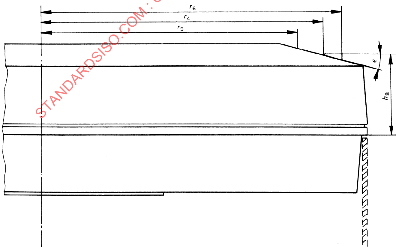
FIGURE 9 — Partial front view of the removable cover in the working position
