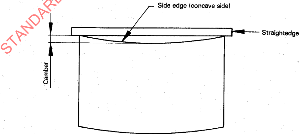
Figure 2 — Measurement of camber
