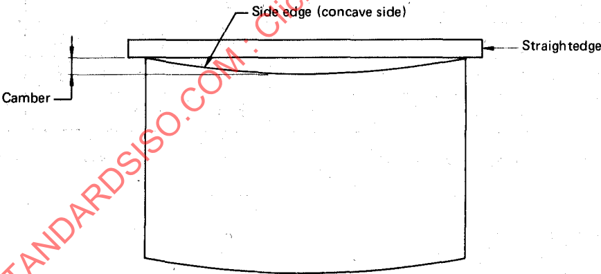
FIGURE 1 — Measurement of camber
