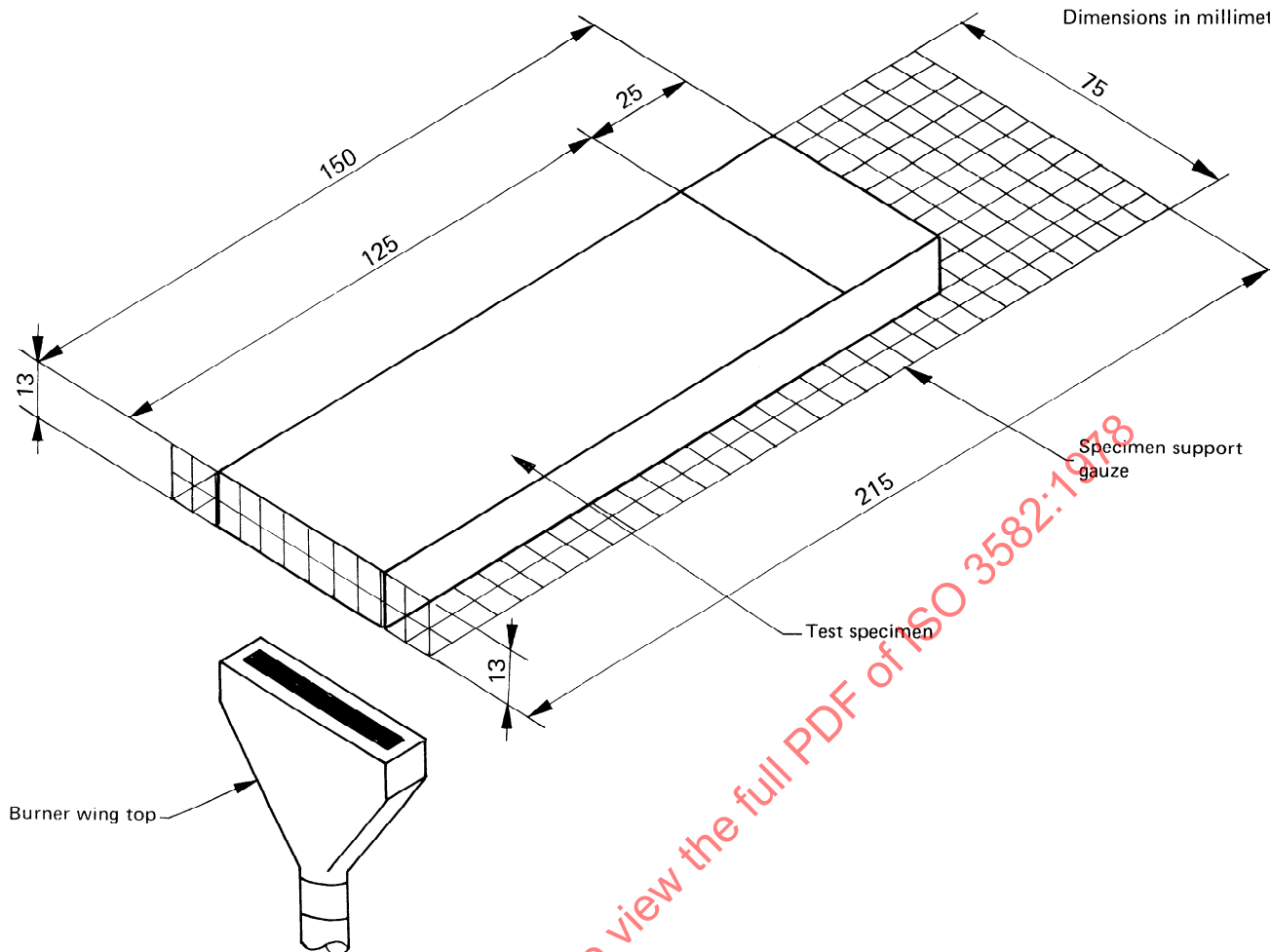
FIGURE 3 — Test specimen and specimen support gauze (5.4)
