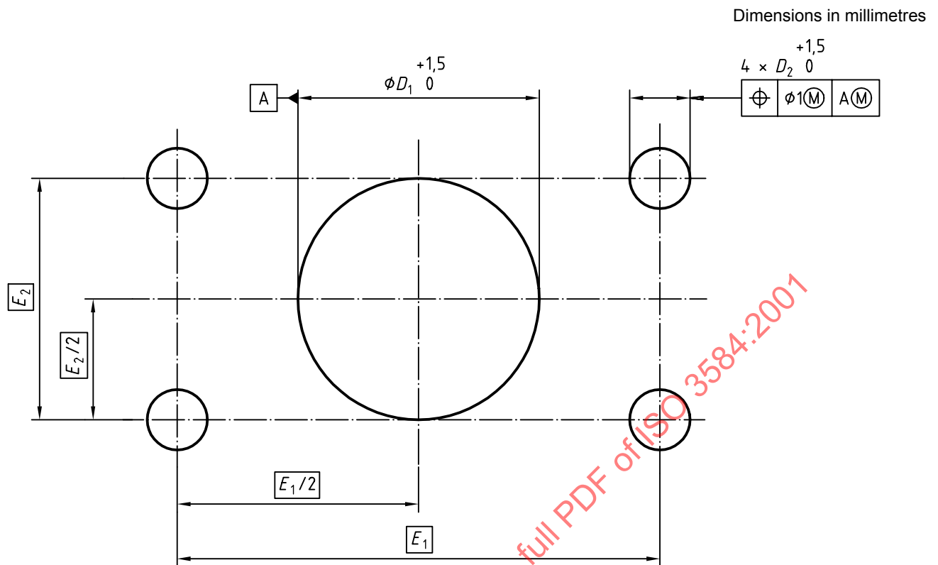
Figure 1 — Drilling pattern
