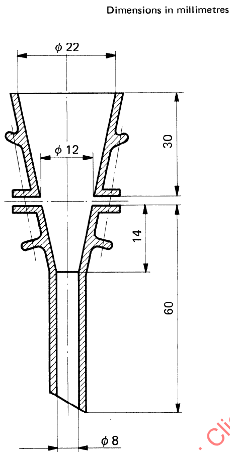
FIGURE 1 — Micro-filtering device
