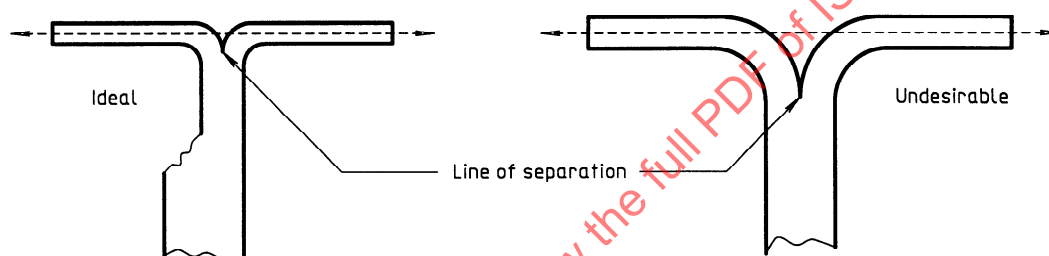
Figure 1 — Position of line of separation of plies
