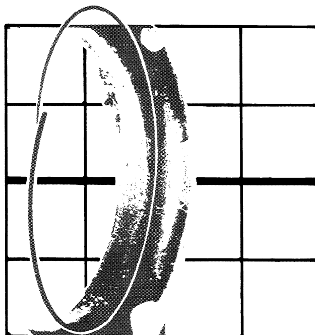
Figure 4 — Parting line indentation
