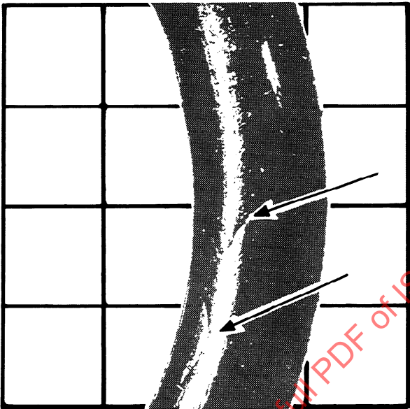
Figure 5 — Flow marks
