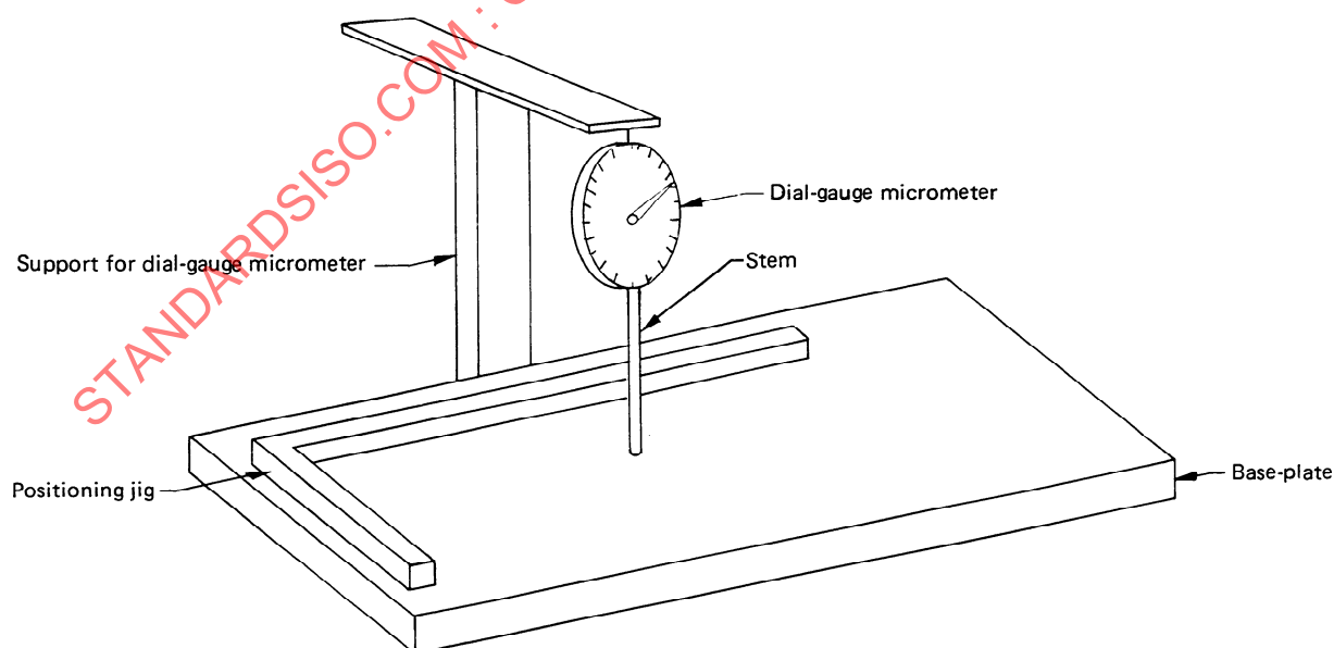
FIGURE 1 – Stand for supporting test specimens and dial-gauge micrometer
