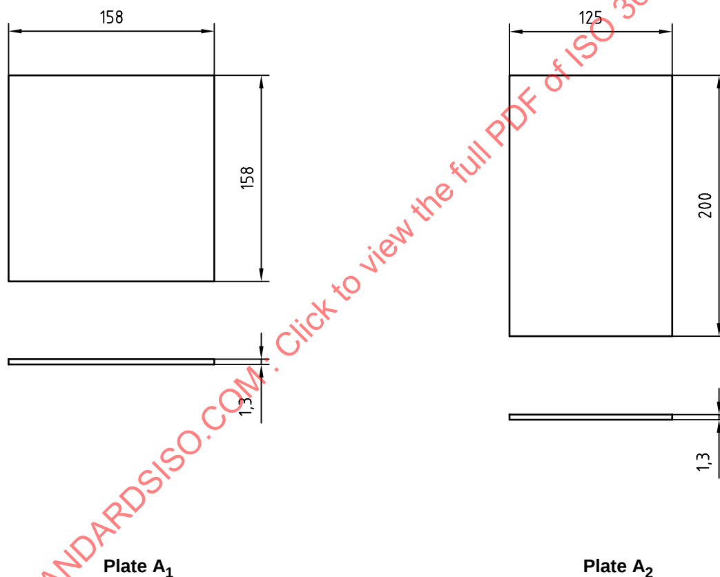
Figure 2 — Light mild-steel plate (density of steel 7,84 Mg/m 3 ) for determination of average thickness
