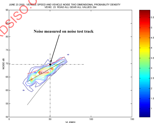
Figure A.20 — Maximum level of noise emitted by vehicle in urban driving conditions at the maximum acceleration (density of probability along the trip)
