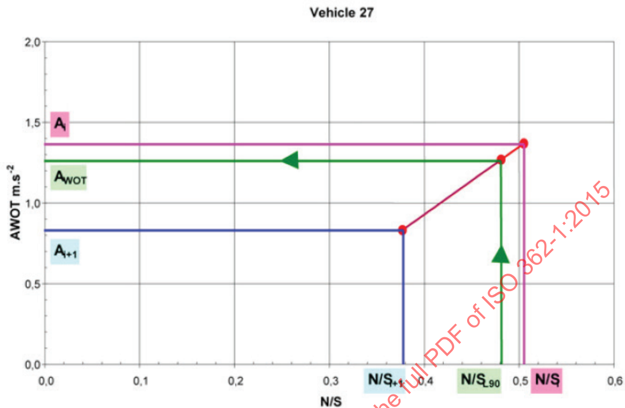
Figure A.16 — Determination of wide-open-throttle acceleration a_{wot\ 50}
