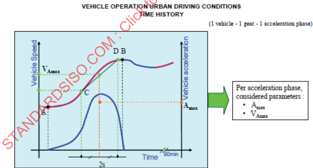
Figure A.3 — Maximum acceleration definition
