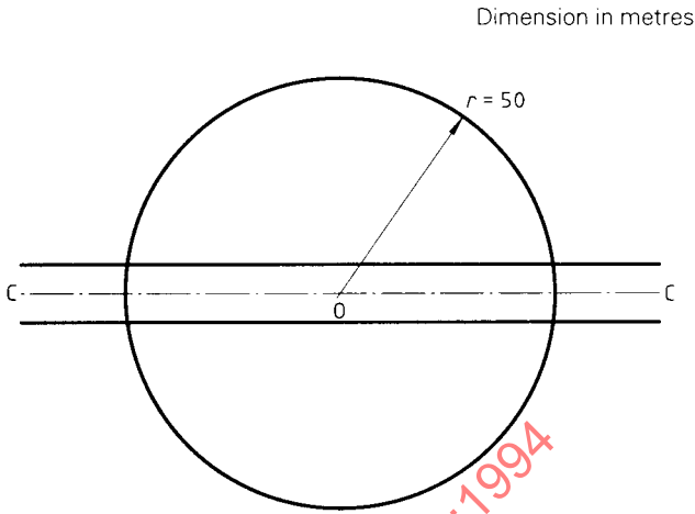
Figure 1 — Test site
