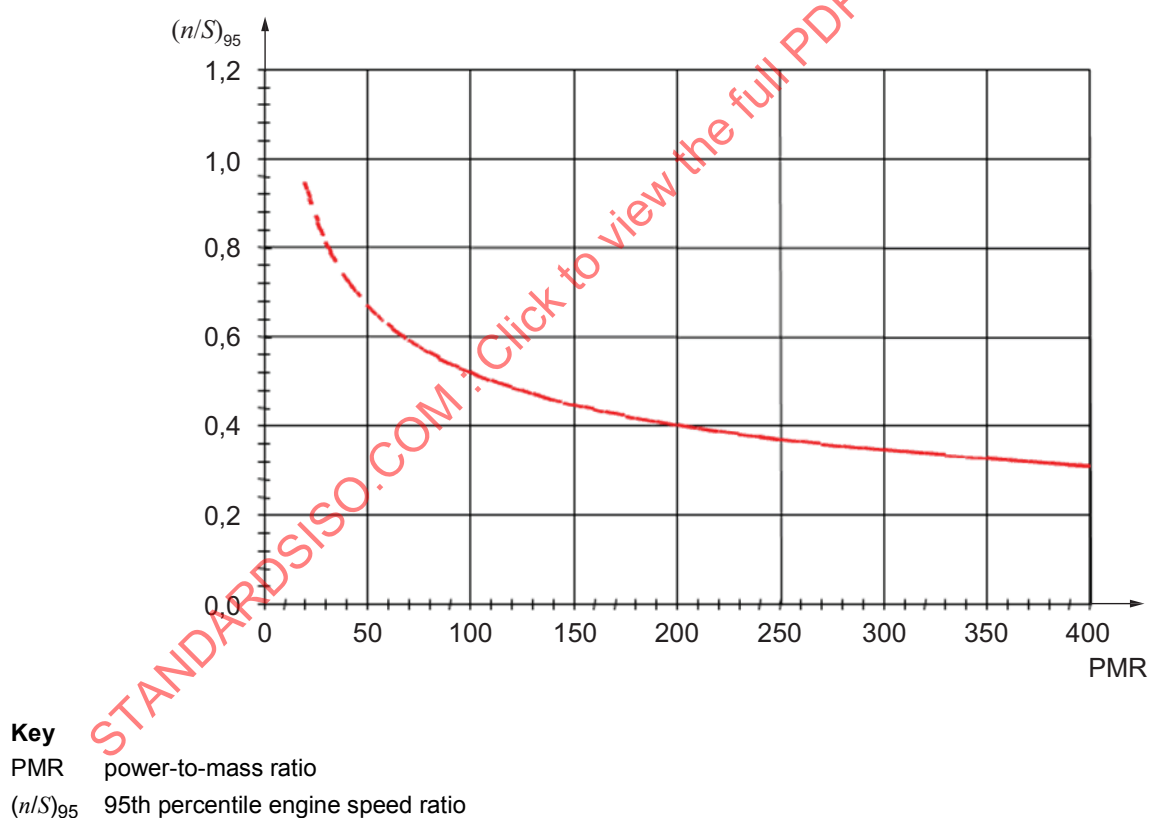
Figure A.1 — Regression curve (n/S)_{95} = f(\text{PMR})
