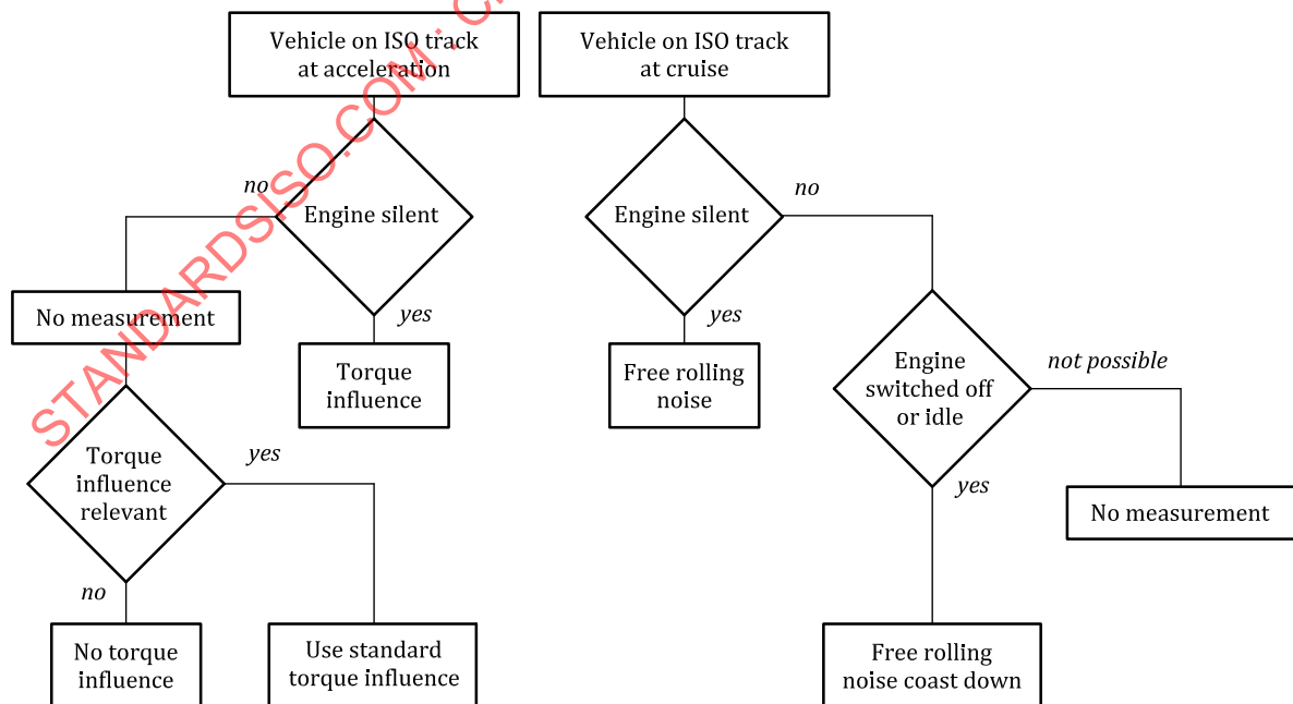
Figure B.7 — Example for a procedure for checking which method to use
