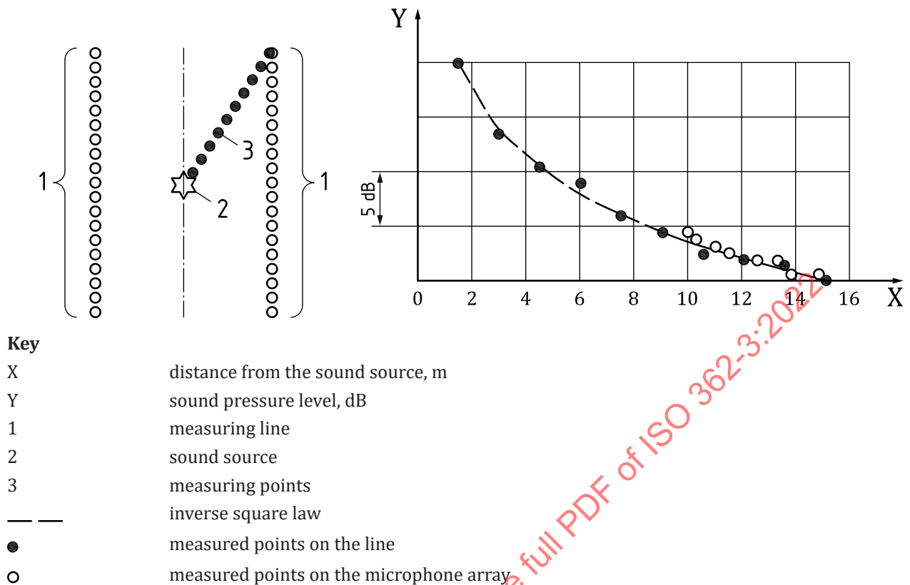
Figure 5 — Example of validation according to 7.3.2.3
