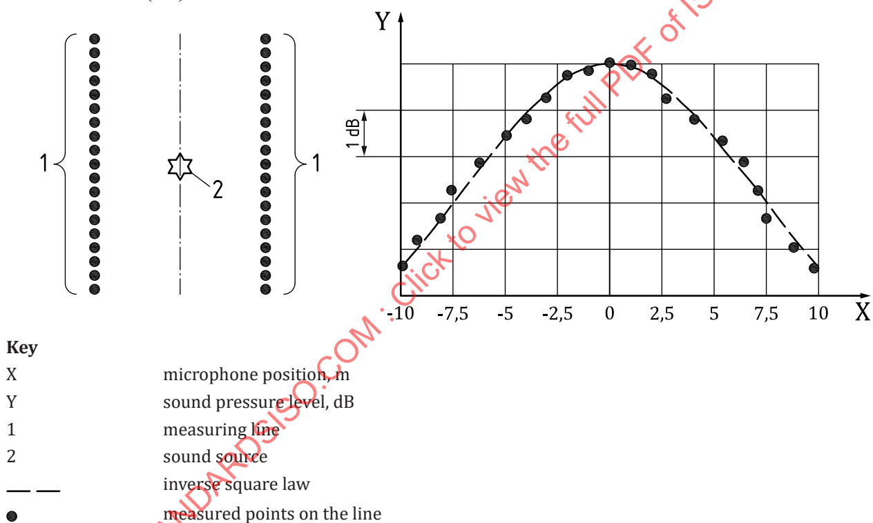
Figure 6 — Example of validation according to 7.3.2.4
