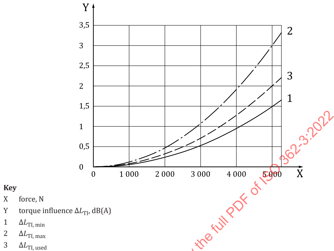
Figure B.6 — Example for standard function torque influence
