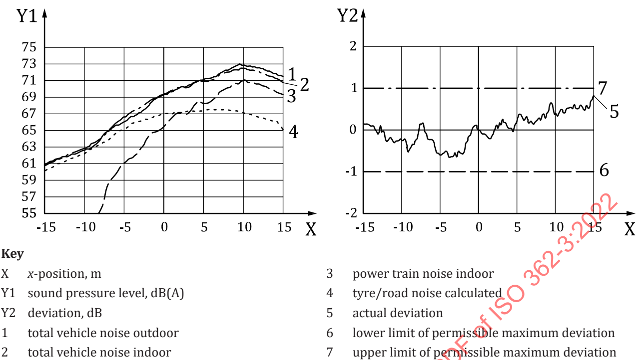
Figure A.3 — Example of an indoor/outdoor validation with indication of the permissible maximum deviation
