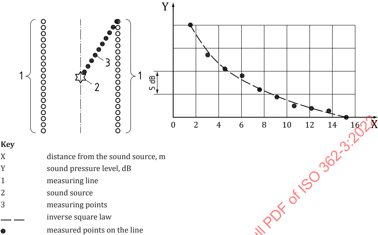
Figure 4 — Example of validation according to 7.3.2.2
