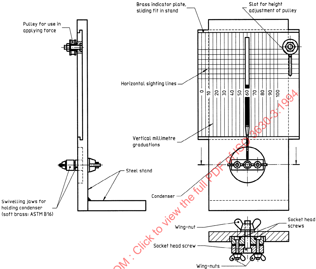
Figure 6 — Apparatus for resistance to bend testing, hand type
