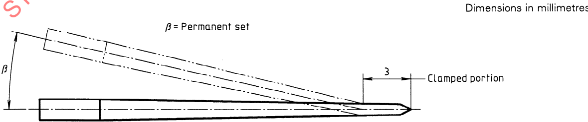
Figure 5 — Measurement of permanent set
