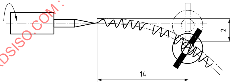
Figure 5 — Apparatus for testing resistance to fatigue — Type 2 instruments
