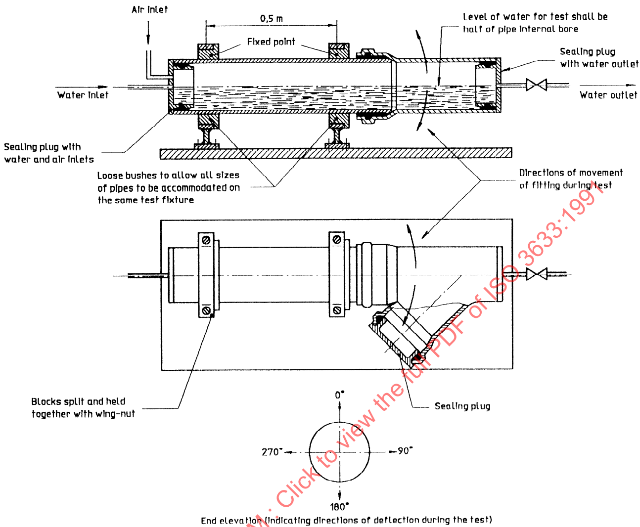
Figure C.1 — Test assembly for airtightness test
