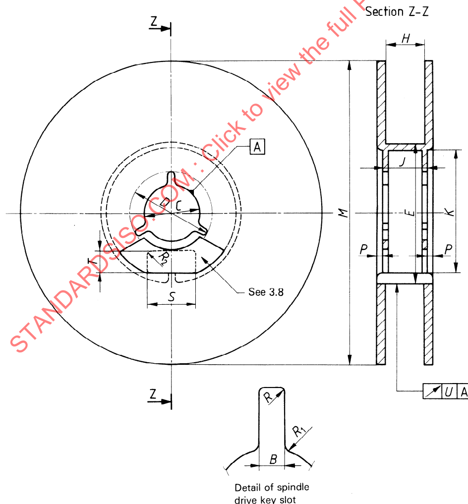
Figure 1 — Reel/spool dimensions
