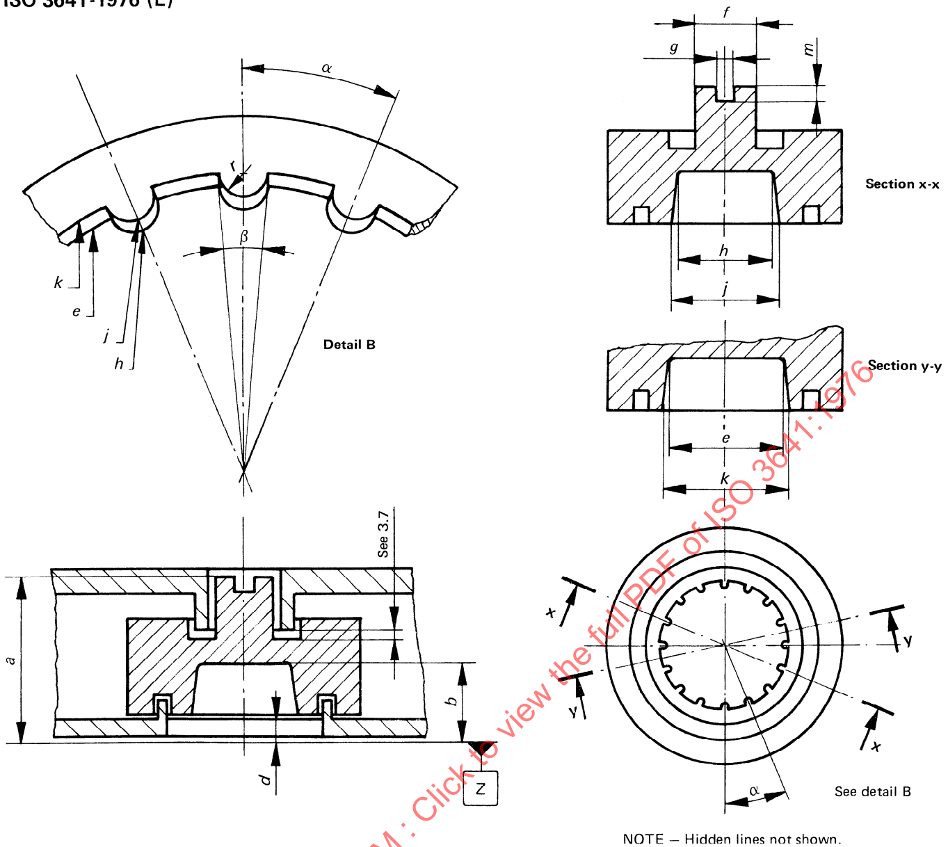
FIGURE 2 — Section of cartridge containing core (see 3.6)
