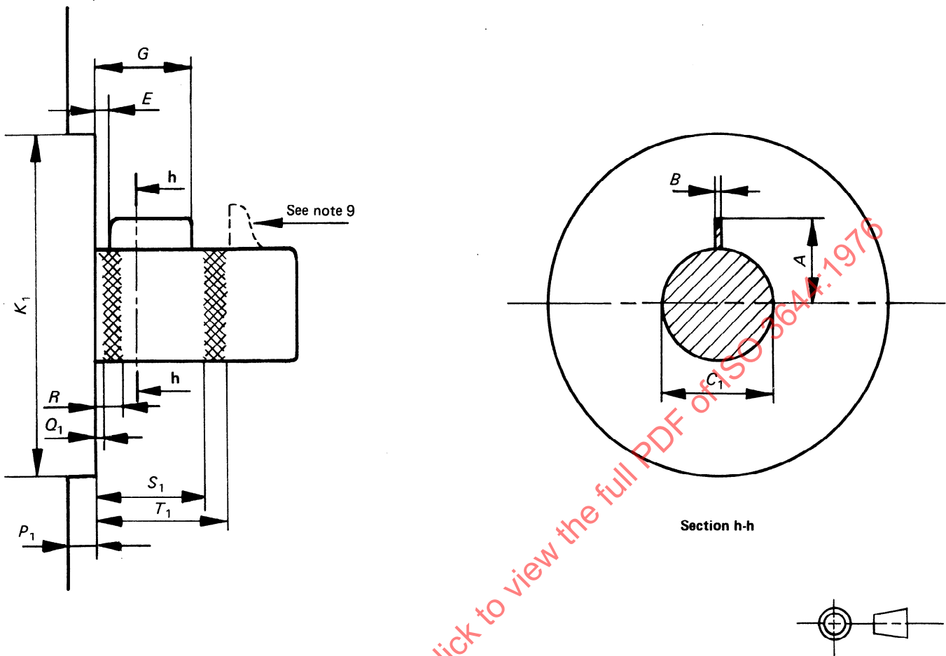
FIGURE 3 — Projector spindle
