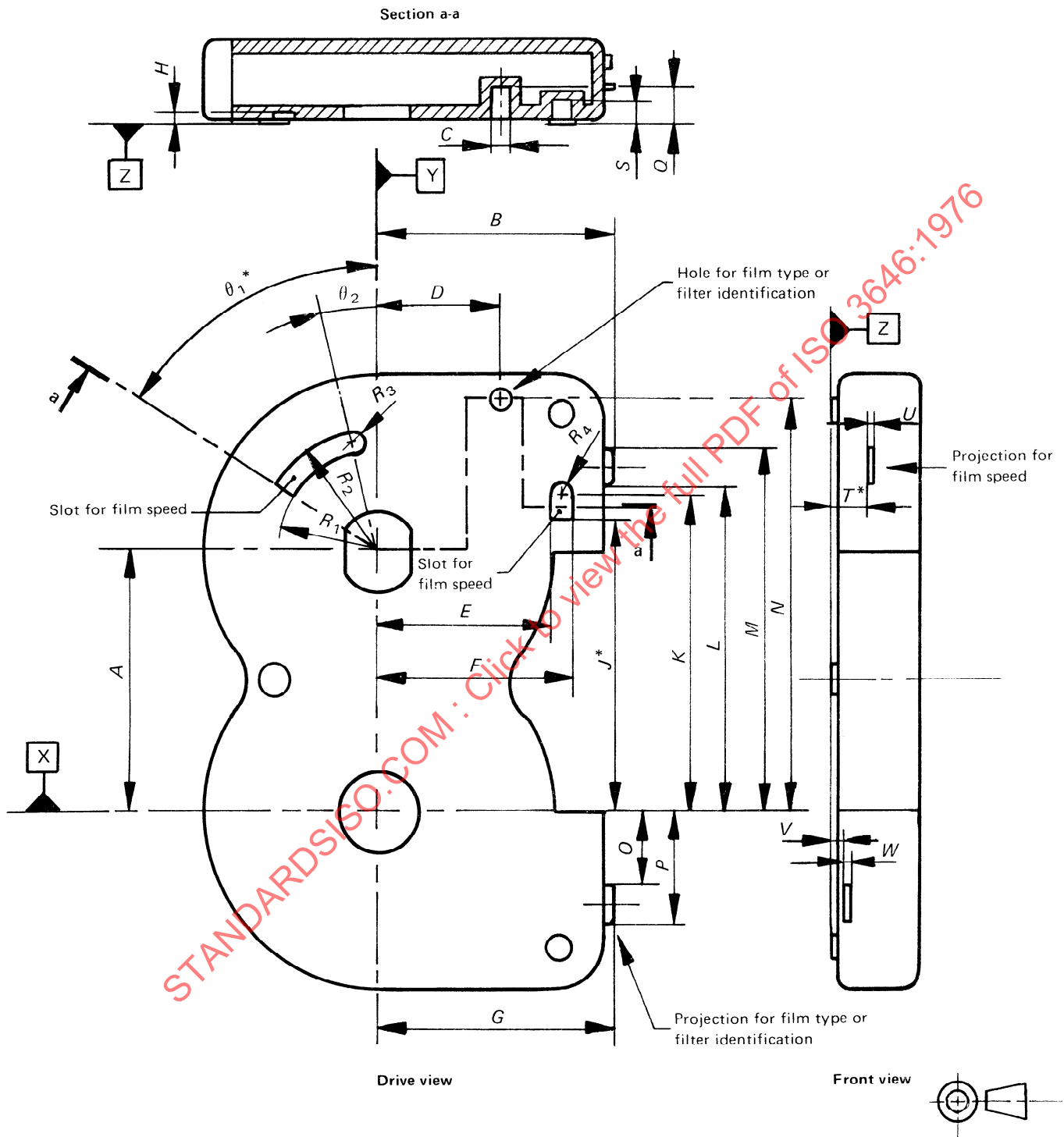
FIGURE 1 — Location and dimensions of slots, projections and hole
