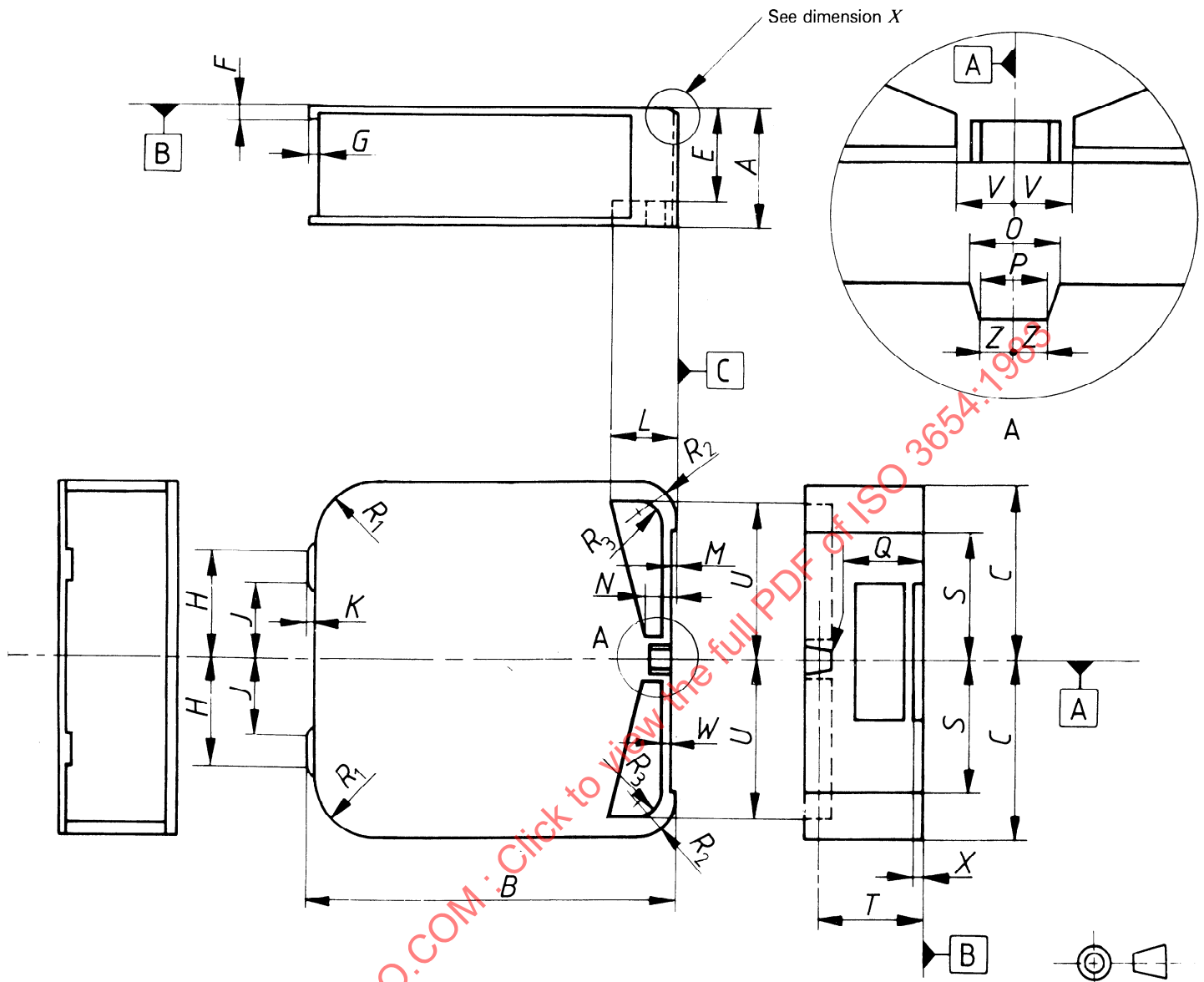
Figure 1 — External cartridge camera fit characteristics
