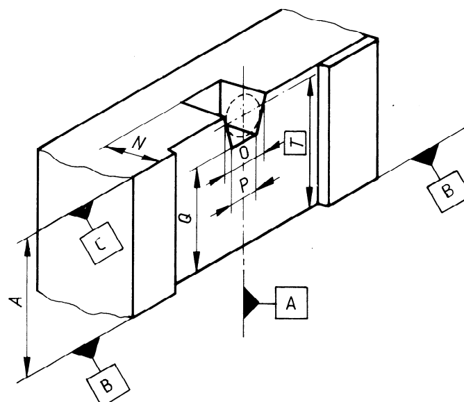
Figure 2 — Camera-locating slot
