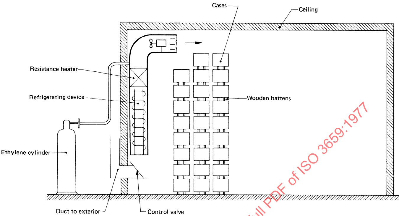
FIGURE 1 – Diagram of ripening room
