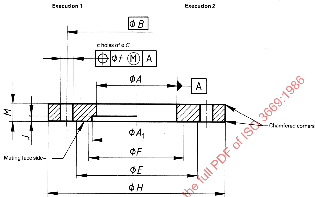
Figure 1 — Preferred series of flanges
