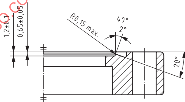
Figure 2 — Knife-edge detail
