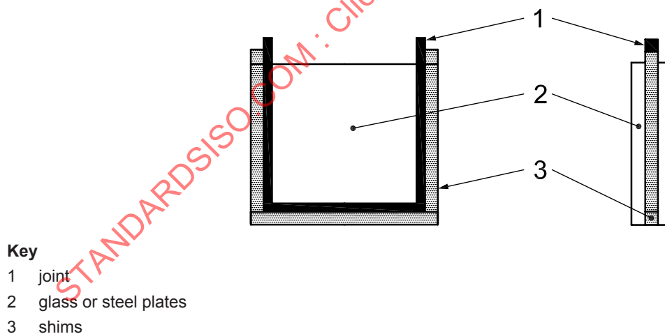
Figure 1 — Apparatus for preparing test sheets
