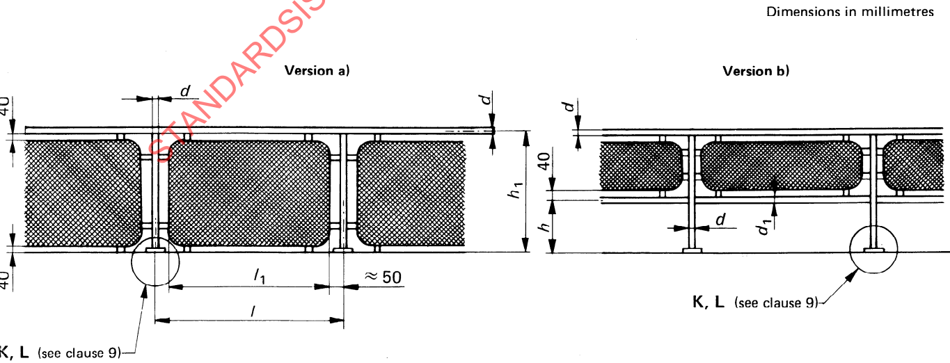
FIGURE 2 — Diagram of network deck rail
