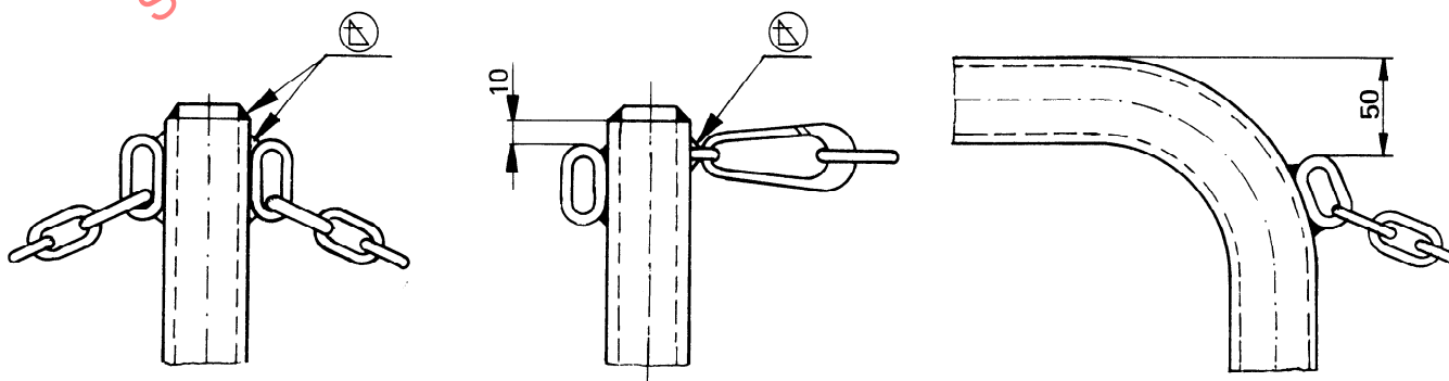
FIGURE 4 — Methods of fixing the chains on stanchions and handrail
