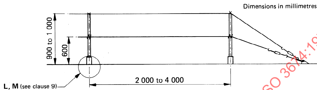
FIGURE 5 — Diagram of rope deck rail
