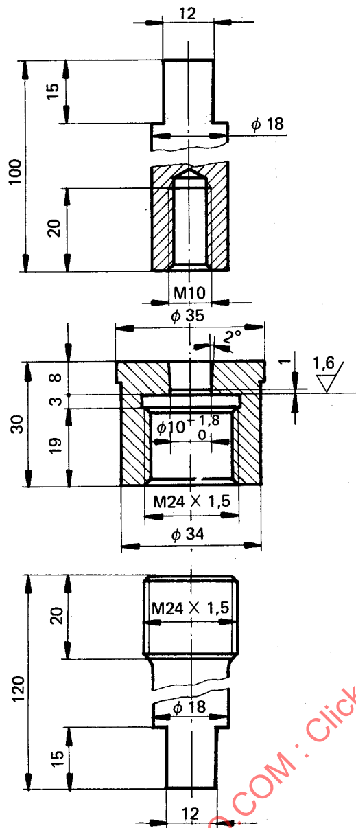
FIGURE 5 — Fixture for tensile loading, Type II test pieces
