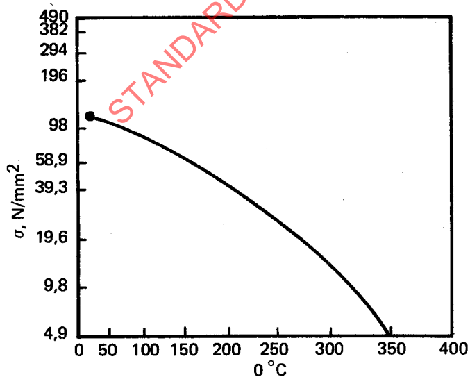
FIGURE 6 – Typical curve of instantaneous hot shearing strength
