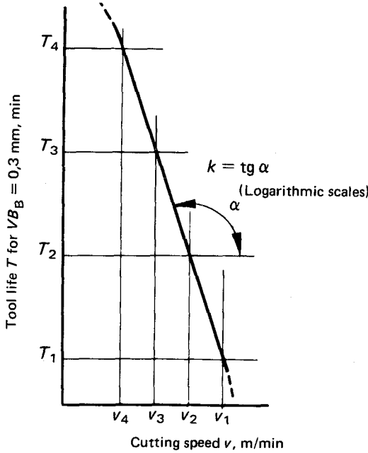
FIGURE 11 — v - T curve for VB_B = 0,3 mm
