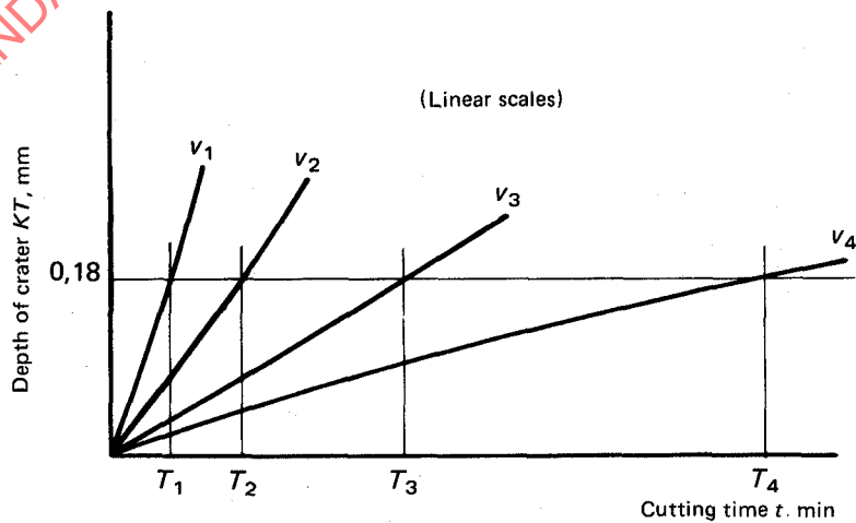
FIGURE 10 – Development of crater depth for different cutting speeds
