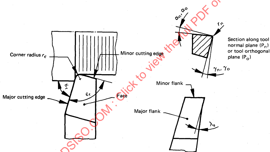
FIGURE 1 — Illustration of tool angles
