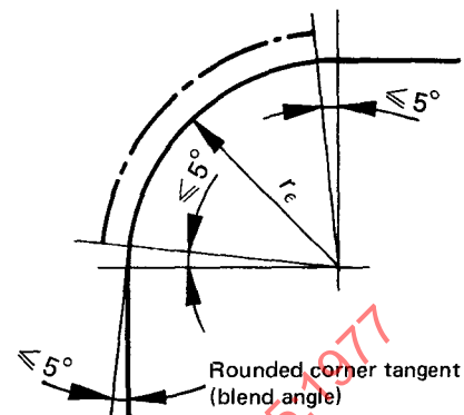
FIGURE 2 — Details of rounded corner
