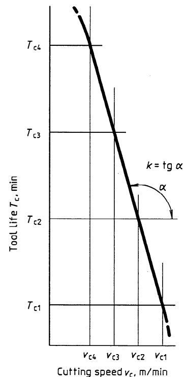
Figure 12 — v_c – T_c curve based on figure 10 (Logarithmic scales)
