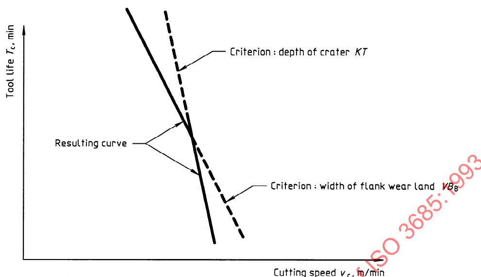
Figure 7 — Broken v_c - T_c curve, combined flank and crater wear (Logarithmic scales)
