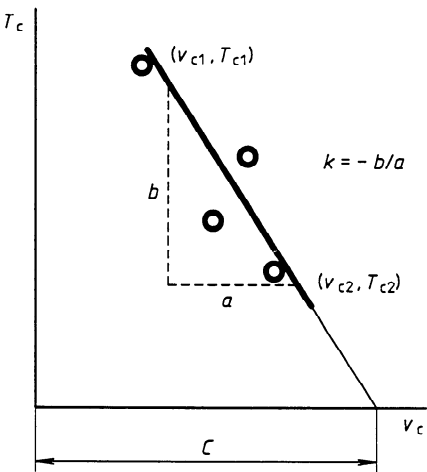
Figure F.1 — (Logarithmic scales)
