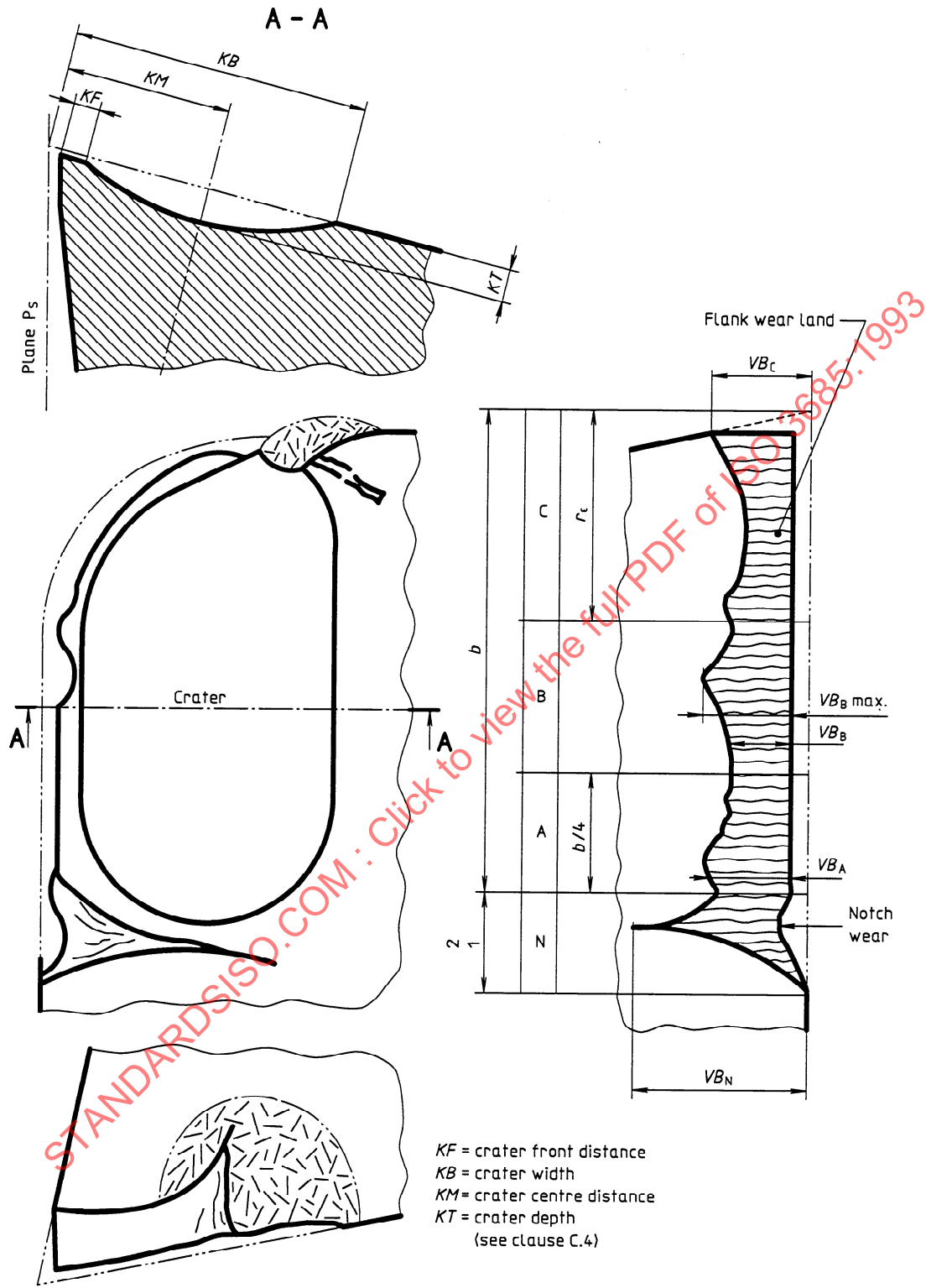
Figure 8 — Some types of wear on turning tools
