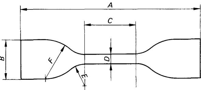
FIGURE 1 — Die
