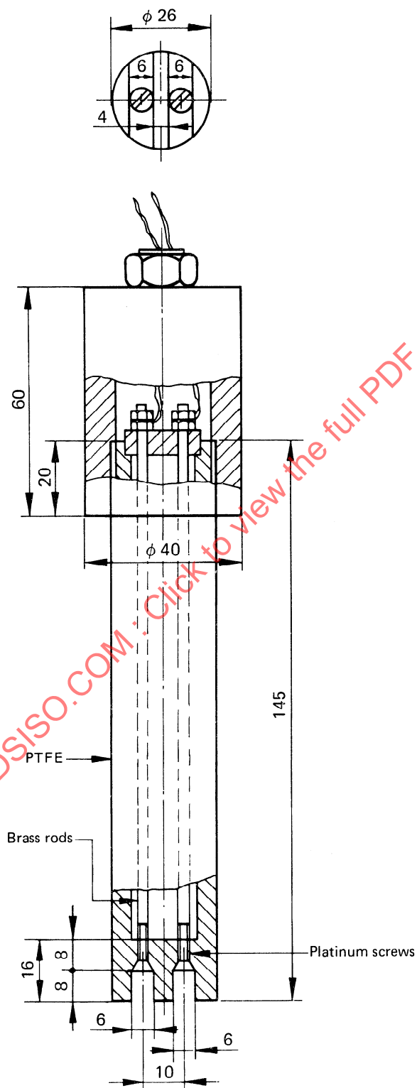
Figure 2 — Dip cell electrode
